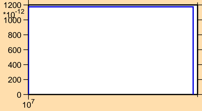
\sigma vs. E for ^{121}\text{Xe} (mt 45)
