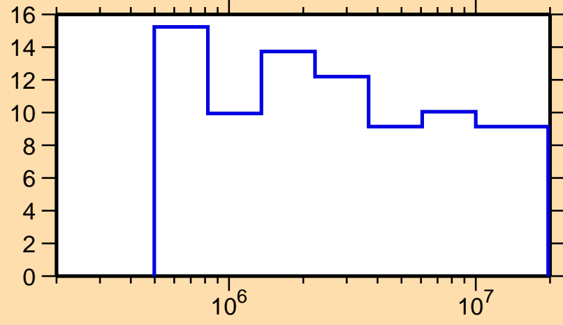
\Delta\sigma/\sigma vs. E for ^{121}\text{Xe}(n,el.)
