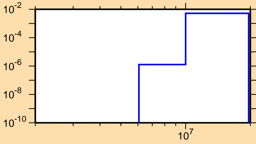
\sigma vs. E for ^{121}\text{Xe}(n,d)
