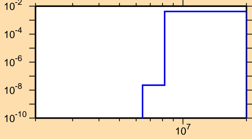
\sigma vs. E for ^{121}\text{Xe}(n,d)
