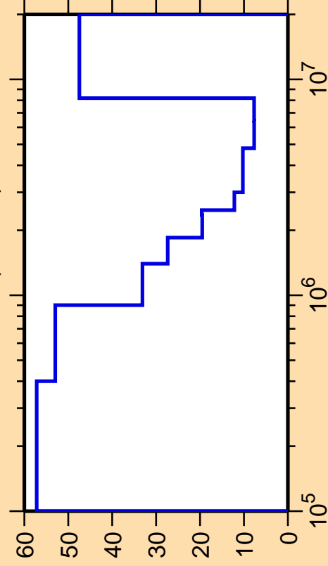
\Delta\sigma/\sigma vs. E for ^{121}\text{Xe}(n,\text{inel.})
