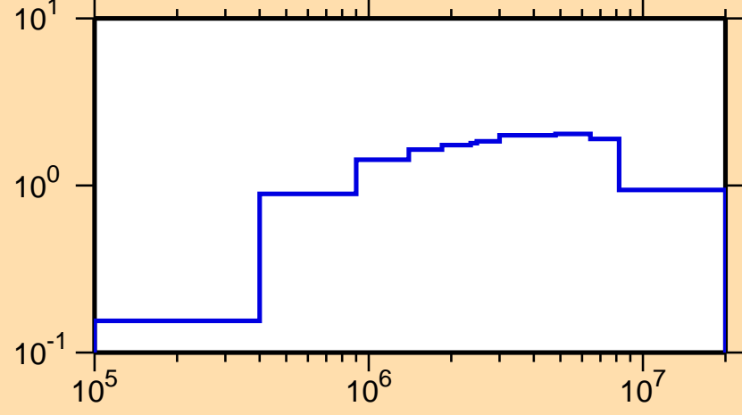
\sigma vs. E for ^{121}\text{Xe}(n,\text{inel.})
