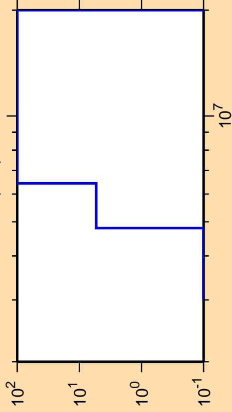
\Delta\sigma/\sigma vs. E for ^{121}\text{Xe}(n,d)
