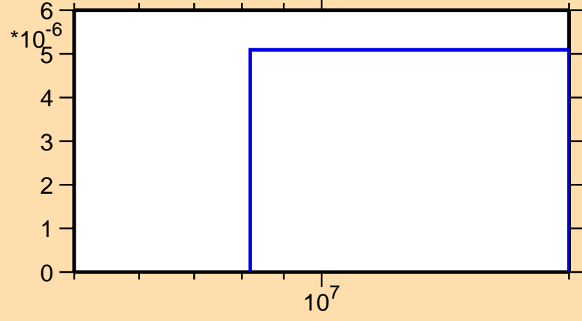
\sigma vs. E for ^{121}\text{Xe}(n,2np)
