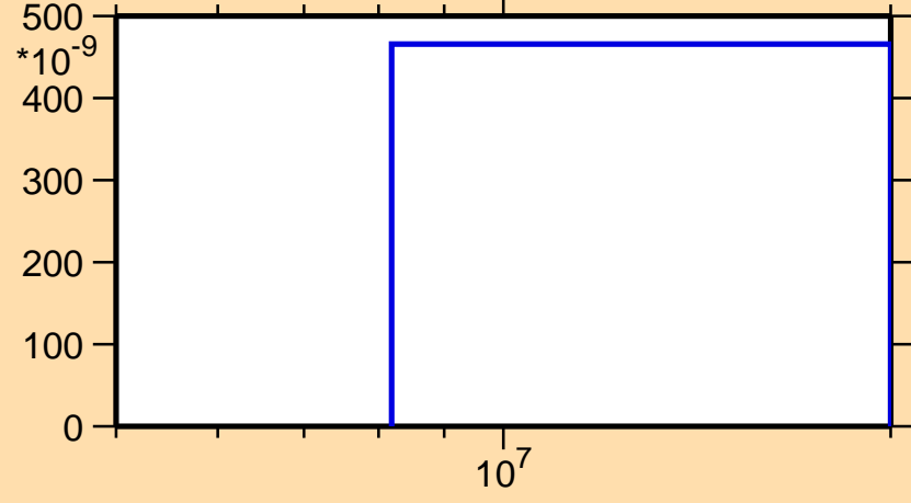
\sigma vs. E for ^{121}\text{Xe}(n,2n\alpha)
