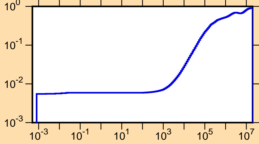
\mu vs. E for ^{123}\text{Xe}(\text{mt251})
