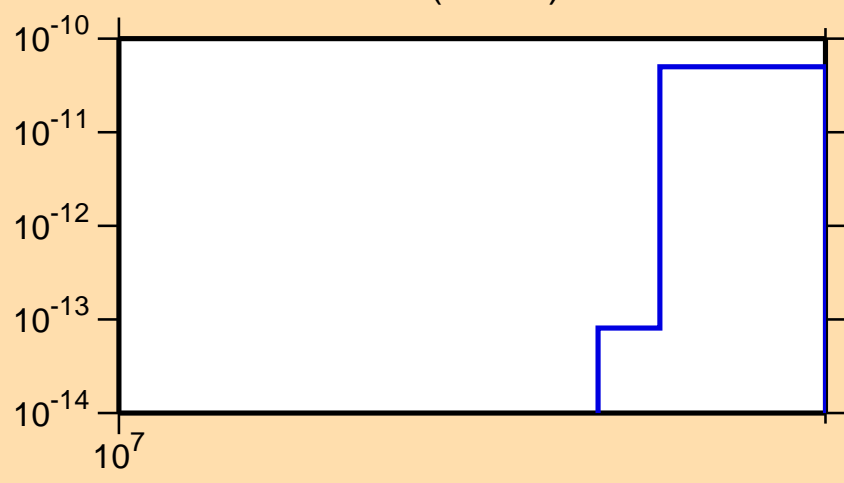
\sigma vs. E for ^{123}\text{Xe}(\text{mt } 34)
