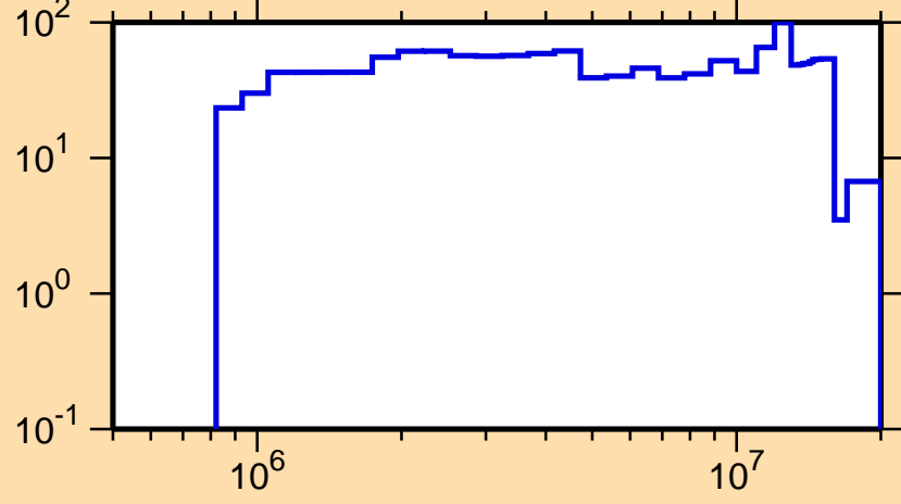
\Delta\sigma/\sigma vs. E for ^{123}\text{Xe}(n,n_1)
