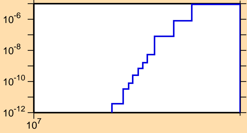
\sigma vs. E for ^{123}\text{Xe}(n,2n\alpha)
