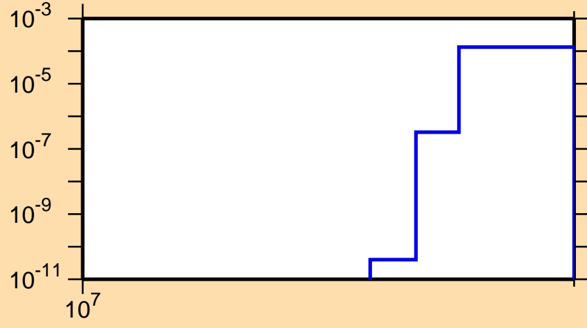
\sigma vs. E for ^{123}\text{Xe}(n,2np)
