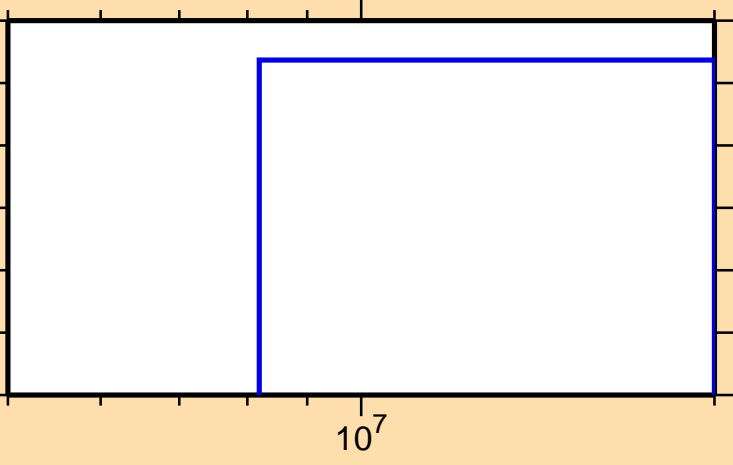
\sigma vs. E for ^{123}\text{Xe}(\text{mt117})
