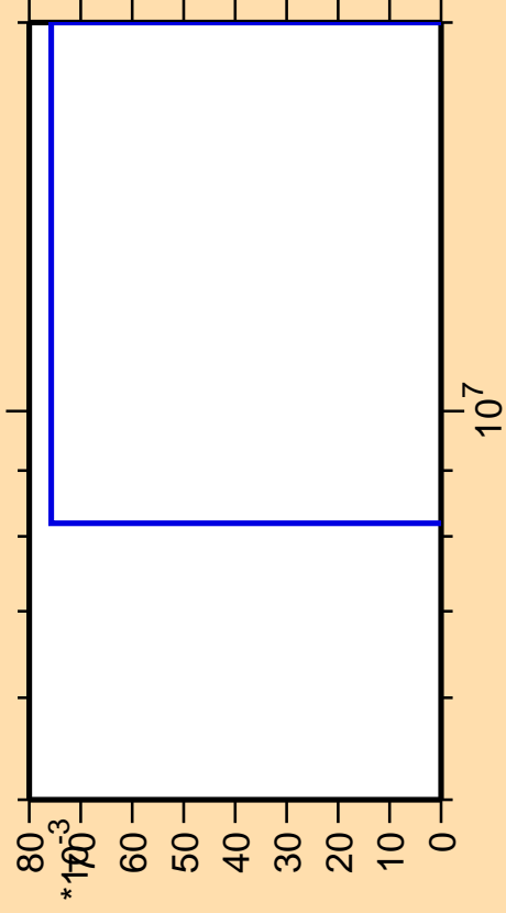
\Delta\sigma/\sigma vs. E for ^{123}\text{Xe}(n,\text{nt})
