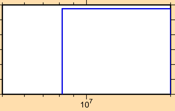
\sigma vs. E for ^{123}\text{Xe}(n,\text{nd})
