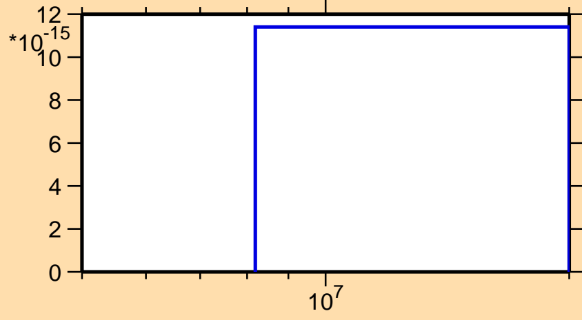
\sigma vs. E for ^{123}\text{Xe}(n,\text{nt})
