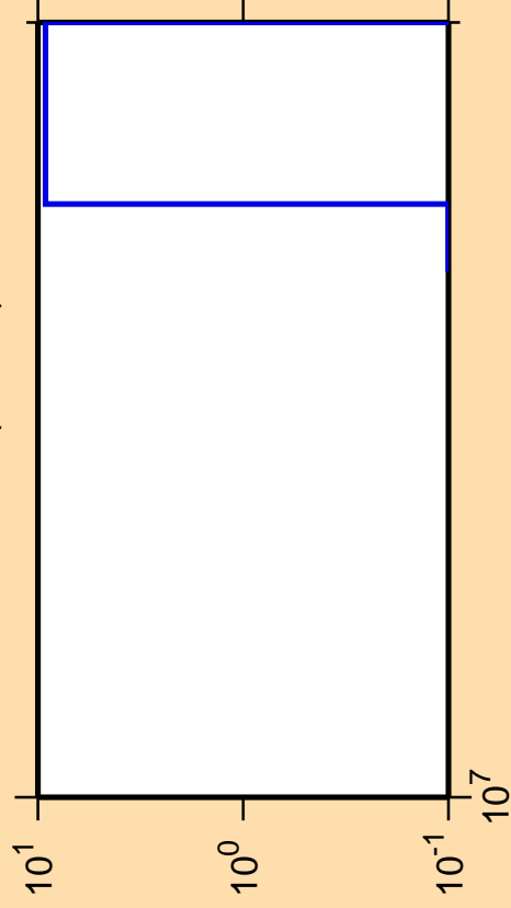
\Delta\sigma/\sigma vs. E for ^{124}\text{Xe} (mt 45)
