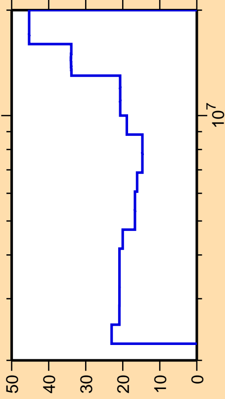
\Delta\sigma/\sigma vs. E for ^{124}\text{Xe}(n,ncont.)
