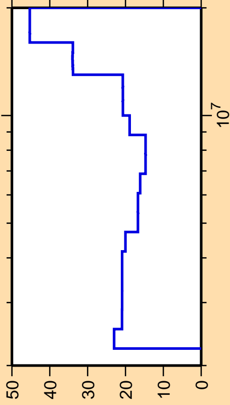
\Delta\sigma/\sigma vs. E for ^{124}\text{Xe}(n,\text{ncont.})
