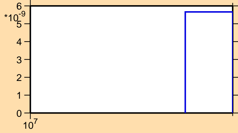
\sigma vs. E for ^{124}\text{Xe}(n,2np)
