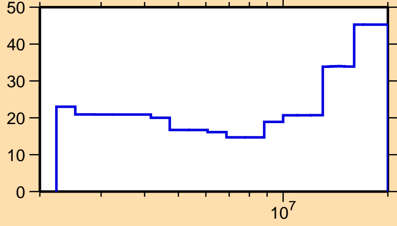
\Delta\sigma/\sigma vs. E for ^{124}\text{Xe}(n,ncont.)
