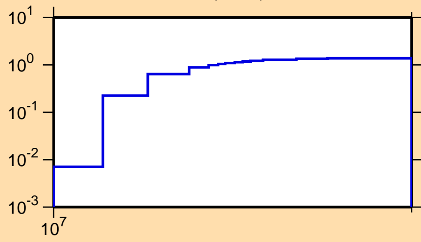
\sigma vs. E for ^{124}\text{Xe}(n,2n)
