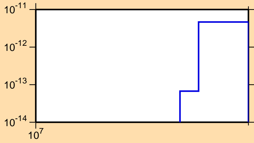
\sigma vs. E for ^{124}\text{Xe}(\text{mt117})
