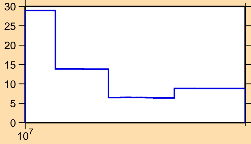
\Delta\sigma/\sigma vs. E for ^{124}\text{Xe}(n,2n)
