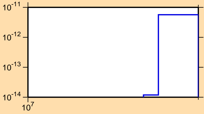
\sigma vs. E for ^{124}\text{Xe} (mt 45)
