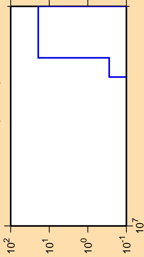
\Delta\sigma/\sigma vs. E for ^{124}\text{Xe}(\text{mt117})
