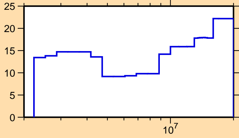
\Delta\sigma/\sigma vs. E for ^{124}\text{Xe}(n,inel.)
