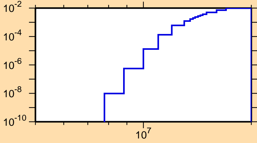
\sigma vs. E for ^{124}\text{Xe}(n,d)
