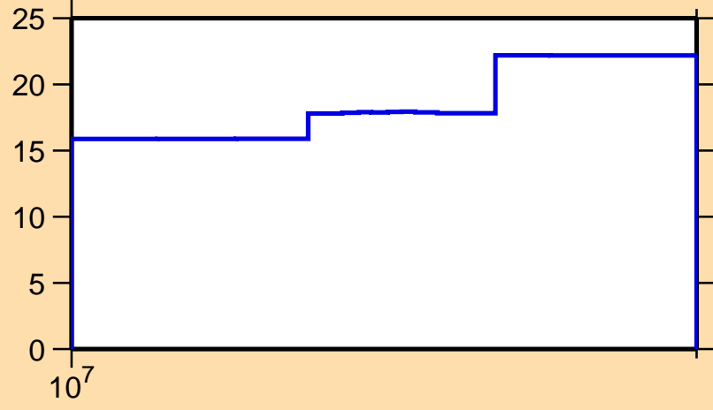
\Delta\sigma/\sigma vs. E for ^{124}\text{Xe}(n,\text{inel.})
