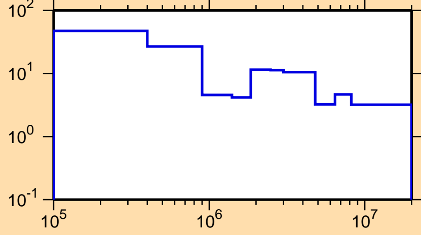
\Delta\sigma/\sigma vs. E for ^{124}\text{Xe}(n,\text{tot.})
