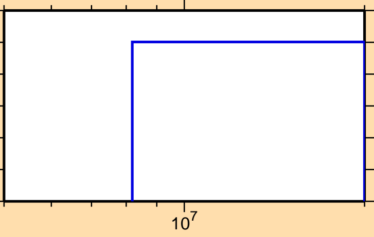
\sigma vs. E for ^{124}\text{Xe}(n,\text{pd})
