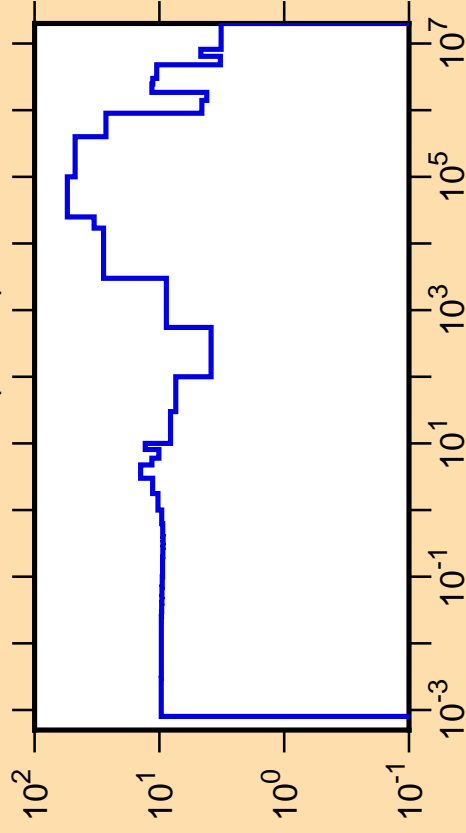
\Delta\sigma/\sigma vs. E for ^{124}\text{Xe}(n,\text{tot.})
