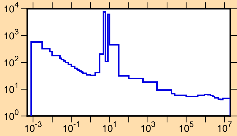
\sigma vs. E for ^{124}\text{Xe}(n,\text{tot.})
