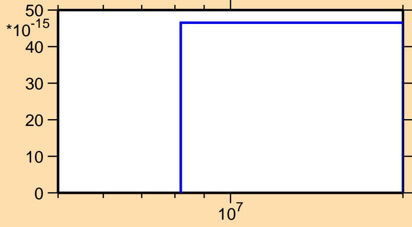
\sigma vs. E for ^{124}\text{Xe}(\text{mt } 45)
