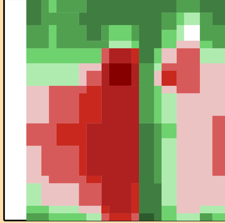
\Delta\sigma/\sigma vs. E for ^{127}\text{Xe}(n,ncont.)
