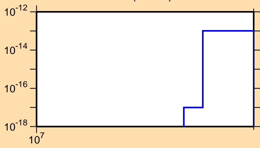
\sigma vs. E for ^{127}\text{Xe}(\text{mt } 34)
