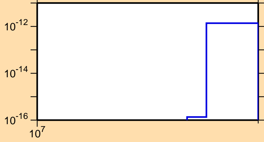
\sigma vs. E for ^{128}\text{Xe}(n,\text{pd})
