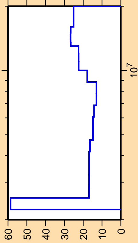
\Delta\sigma/\sigma vs. E for ^{128}\text{Xe}(n,\text{ncont.})
