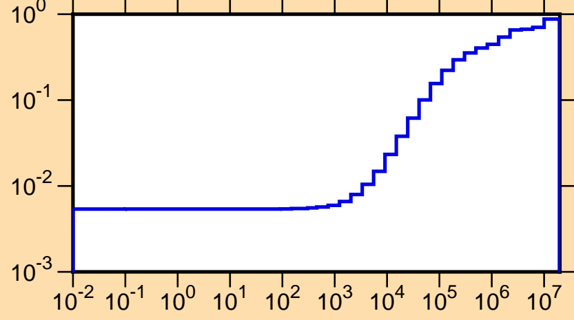
\mu vs. E for ^{128}\text{Xe}(\text{mt251})
