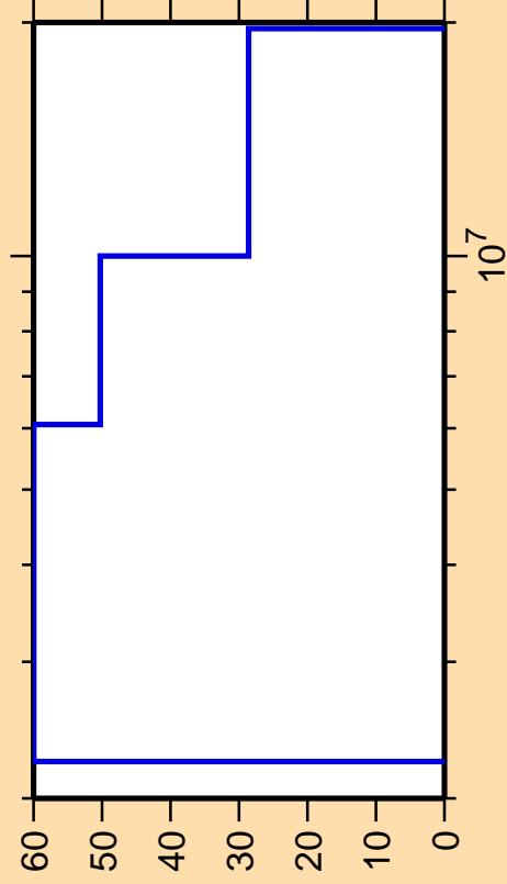
\Delta\sigma/\sigma vs. E for ^{128}\text{Xe}(n,p)
