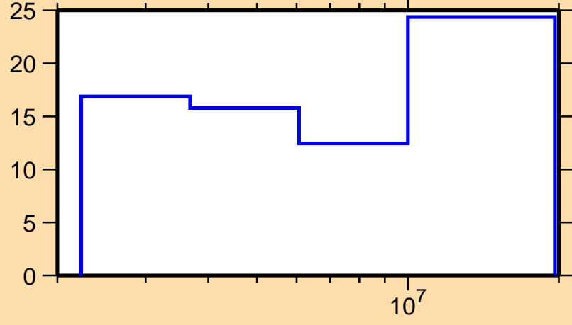
\Delta\sigma/\sigma vs. E for ^{128}\text{Xe}(n,ncont.)
