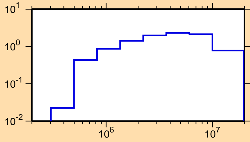
\sigma vs. E for ^{128}\text{Xe}(n,\text{inel.})
