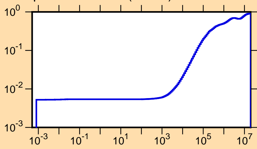
\mu vs. E for ^{129}\text{Xe}(\text{mt251})
