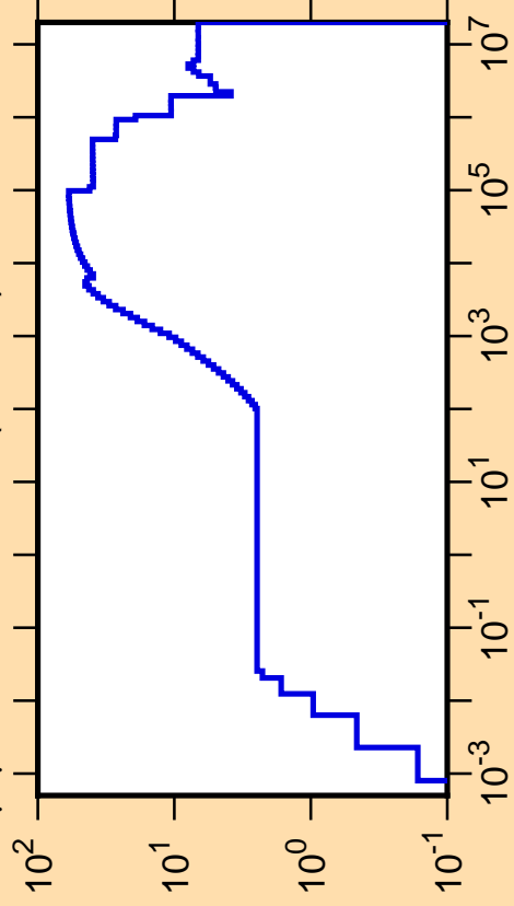
\Delta\mu/\mu vs. E for ^{129}\text{Xe}(\text{mt251})
