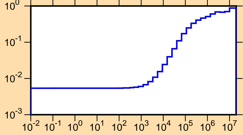
\mu vs. E for ^{129}\text{Xe}(\text{mt251})
