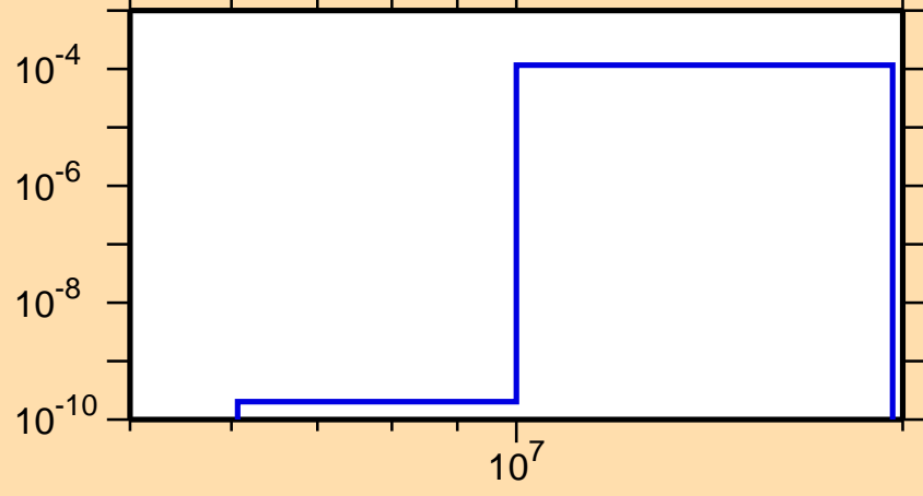
\sigma vs. E for ^{129}\text{Xe}(n,n\alpha)
