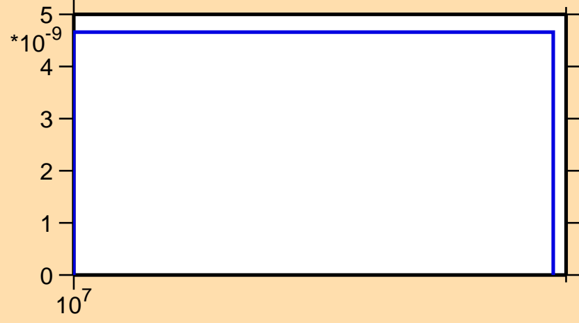
\sigma vs. E for ^{129}\text{Xe}(n,2np)
