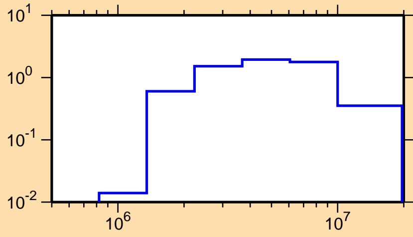
\sigma vs. E for ^{129}\text{Xe}(n,n\text{cont.})
