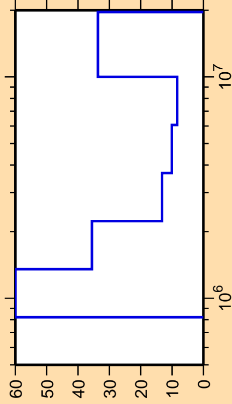
\Delta\sigma/\sigma vs. E for ^{129}\text{Xe}(n,\text{ncont.})
