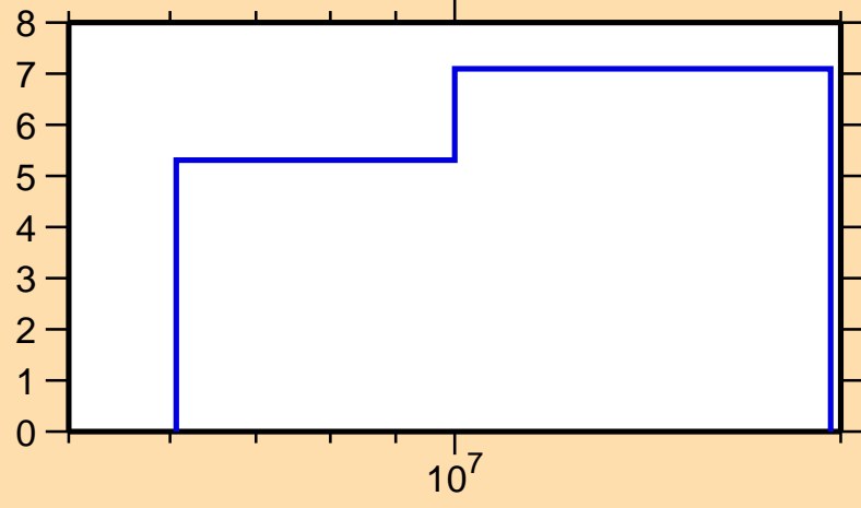
\Delta\sigma/\sigma vs. E for ^{129}\text{Xe}(n,\text{el.})
