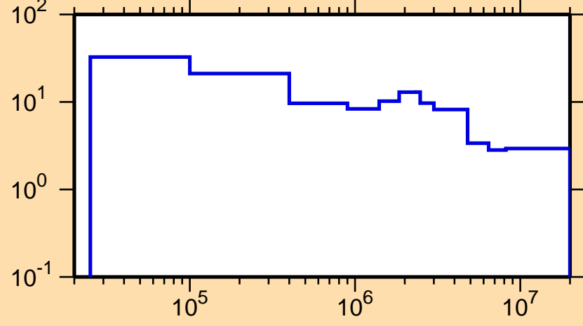
\Delta\sigma/\sigma vs. E for ^{129}\text{Xe}(n,\text{tot.})
