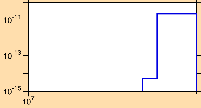
\sigma vs. E for ^{132}\text{Xe}(n,2n\alpha)
