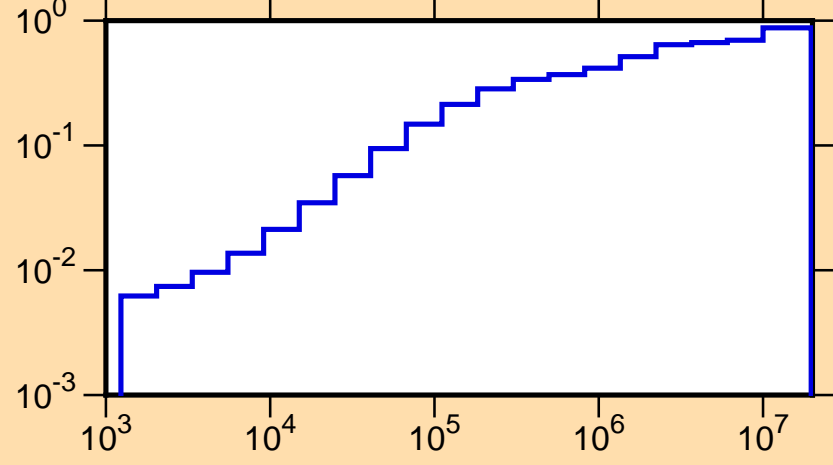
\mu vs. E for ^{132}\text{Xe}(\text{mt251})
