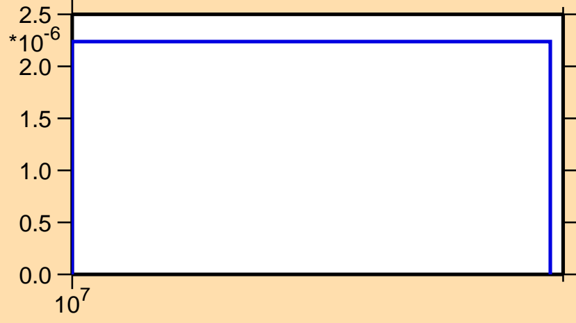
\sigma vs. E for ^{132}\text{Xe}(n,t)
