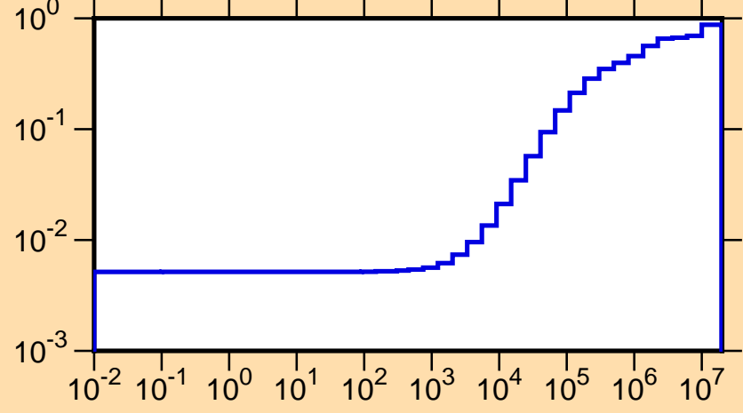
\mu vs. E for ^{133}\text{Xe}(\text{mt251})
