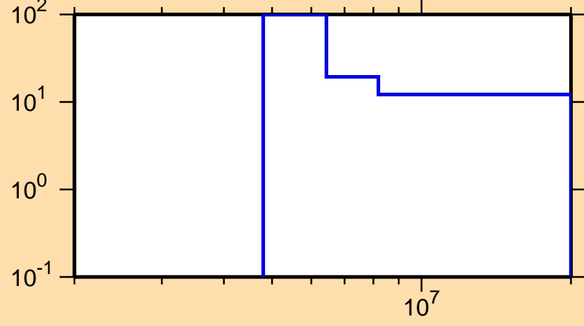
\Delta\sigma/\sigma vs. E for ^{133}\text{Xe}(n,2n)
