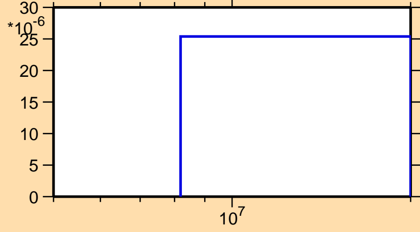
\sigma vs. E for ^{133}\text{Xe}(n,n\alpha)
