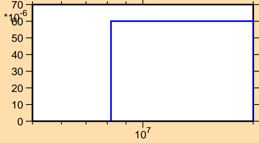
\sigma vs. E for ^{133}\text{Xe}(n,t)
