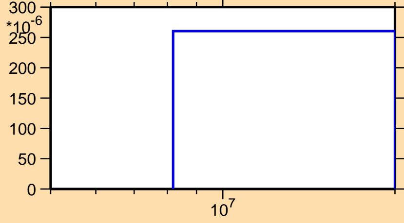
\sigma vs. E for ^{133}\text{Xe}(n,d)
