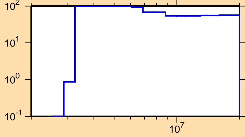
\Delta\sigma/\sigma vs. E for ^{135}\text{Xe}(n,p)
