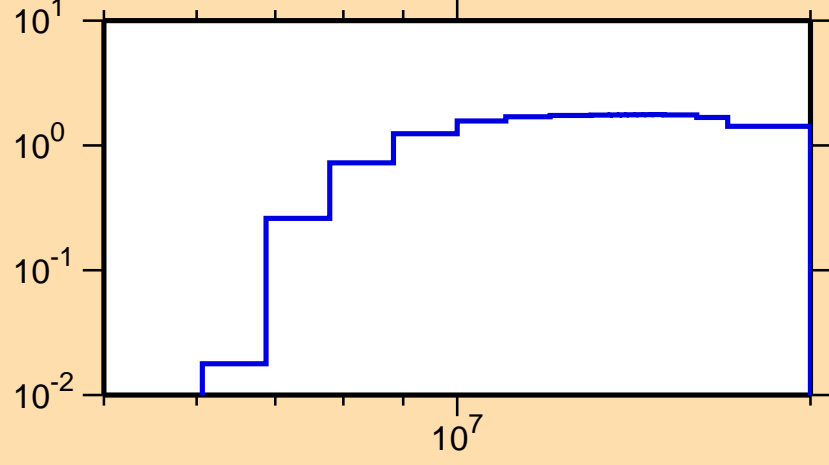
\sigma vs. E for ^{135}\text{Xe}(n,2n)
