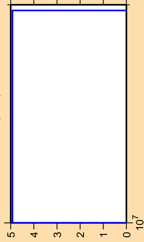
\Delta\sigma/\sigma vs. E for ^{135}\text{Xe}(n,nt)
