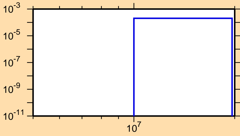
\sigma vs. E for ^{135}\text{Xe}(n,d)
