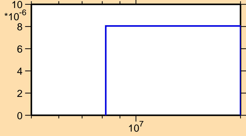
\sigma vs. E for ^{135}\text{Xe}(n,t)
