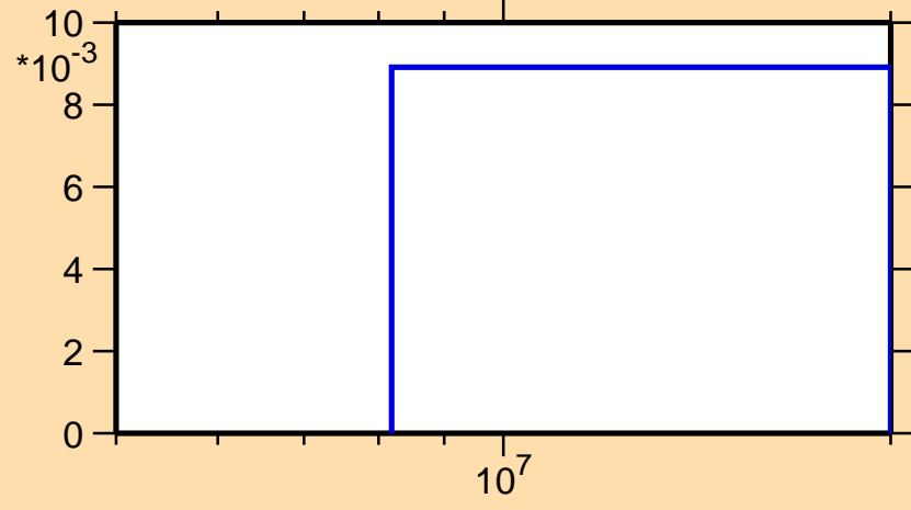
\sigma vs. E for ^{135}\text{Xe}(n,3n)
