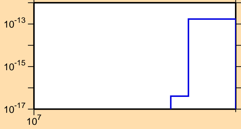
\sigma vs. E for ^{136}\text{Xe}(n,\text{He3})
