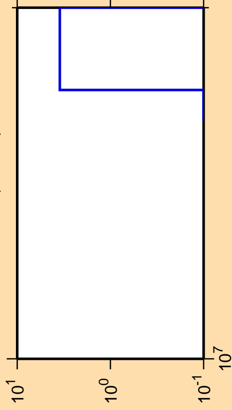
\Delta\sigma/\sigma vs. E for ^{136}\text{Xe}(n,2n\alpha)
