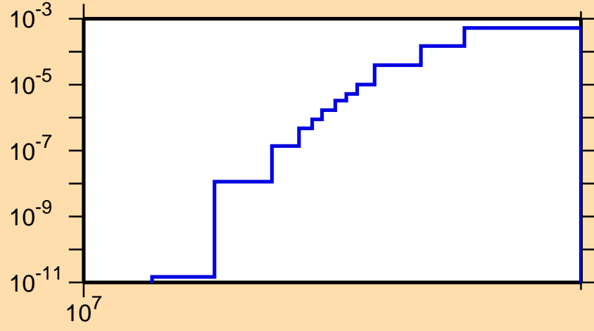
\sigma vs. E for ^{136}\text{Xe}(n,np)
