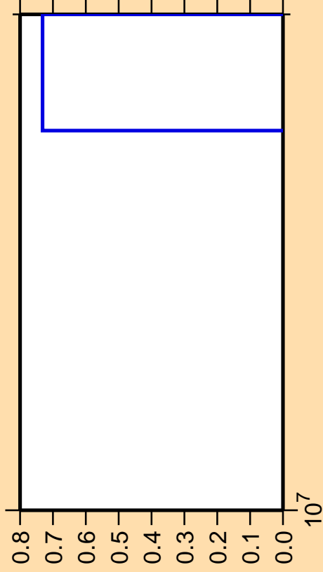
\Delta\sigma/\sigma vs. E for ^{136}\text{Xe}(n,2np)
