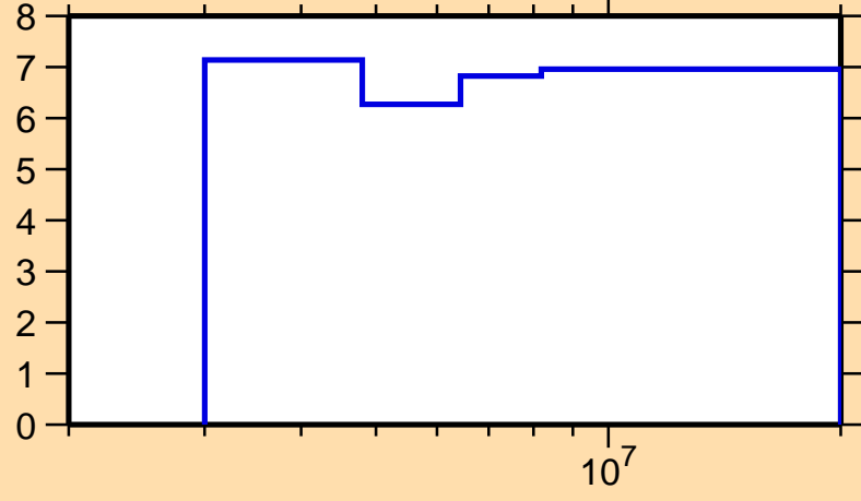
\Delta\sigma/\sigma vs. E for ^{136}\text{Xe}(n,\text{nonel.})
