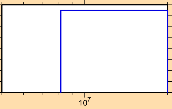
\sigma vs. E for ^{136}\text{Xe}(n,d)
