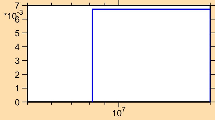
\sigma vs. E for ^{136}\text{Xe}(n,3n)
