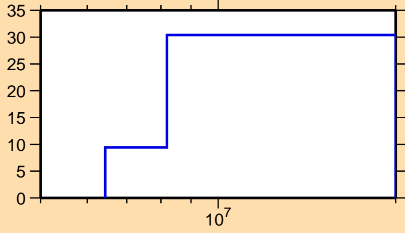
\Delta\sigma/\sigma vs. E for ^{136}\text{Xe}(n,ncont.)
