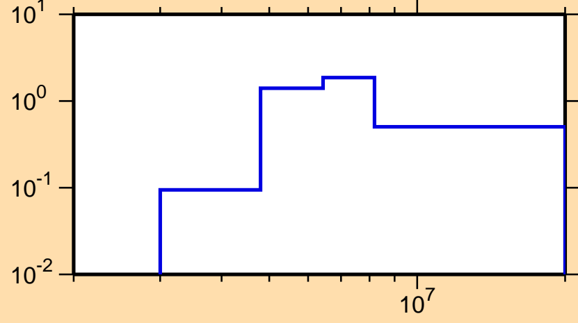
\sigma vs. E for ^{136}\text{Xe}(n,n\text{cont.})
