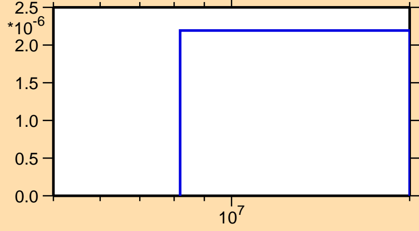
\sigma vs. E for ^{136}\text{Xe}(n,t)
