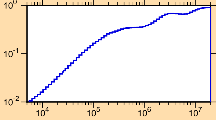
\mu vs. E for ^{137}\text{Xe}(\text{mt251})
