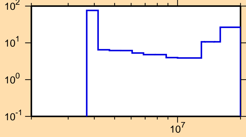
\Delta\sigma/\sigma vs. E for ^{137}\text{Xe}(n,2n)
