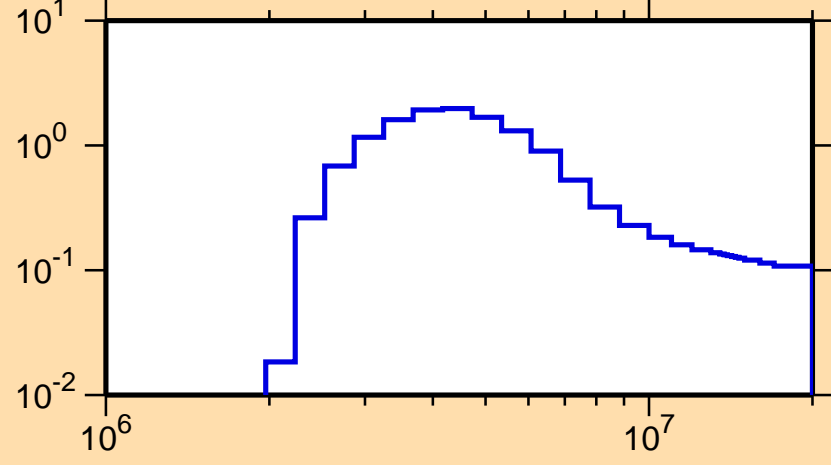
\sigma vs. E for ^{137}\text{Xe}(n,n\text{cont.})
