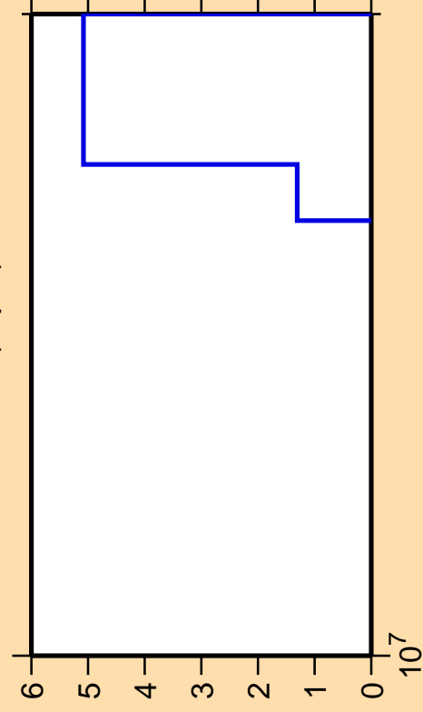
\Delta\sigma/\sigma vs. E for ^{137}\text{Xe}(n,p\alpha)
