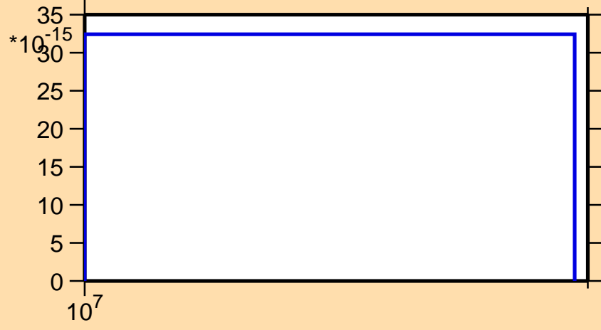
\sigma vs. E for ^{137}\text{Xe}(n,p\alpha)
