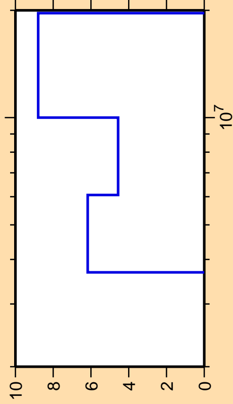
\Delta\sigma/\sigma vs. E for ^{137}\text{Xe}(n,2n)
