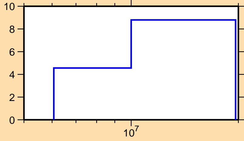
\Delta\sigma/\sigma vs. E for ^{137}\text{Xe}(n,2n)
