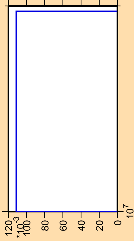
\Delta\sigma/\sigma vs. E for ^{137}\text{Xe}(n,p\alpha)
