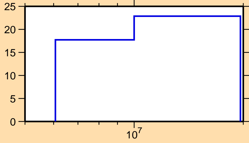
\Delta\sigma/\sigma vs. E for ^{137}\text{Xe}(n,ncont.)
