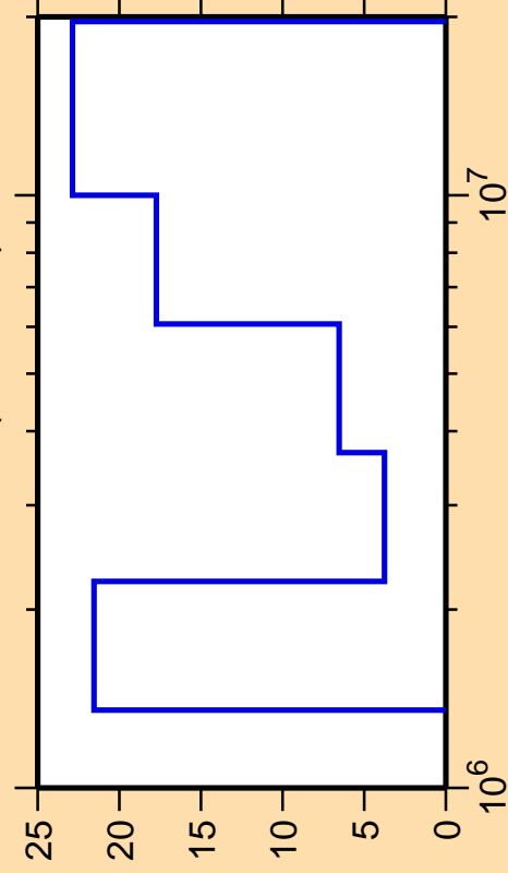
\Delta\sigma/\sigma vs. E for ^{137}\text{Xe}(n,\text{ncont.})
