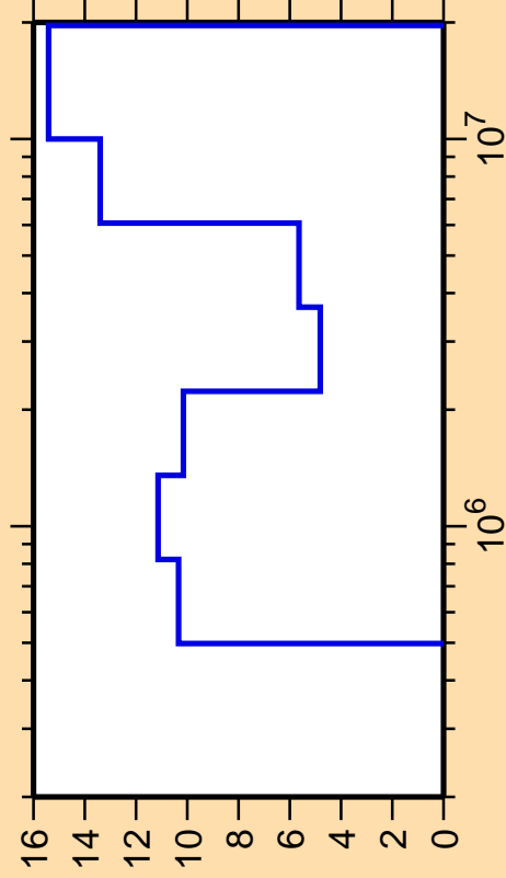
\Delta\sigma/\sigma vs. E for ^{137}\text{Xe}(n,\text{inel.})
