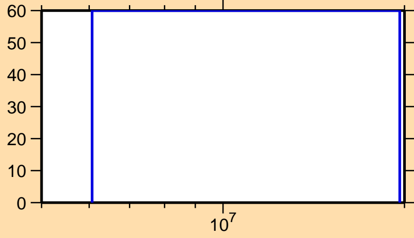
\Delta\sigma/\sigma vs. E for ^{137}\text{Xe}(n,p)
