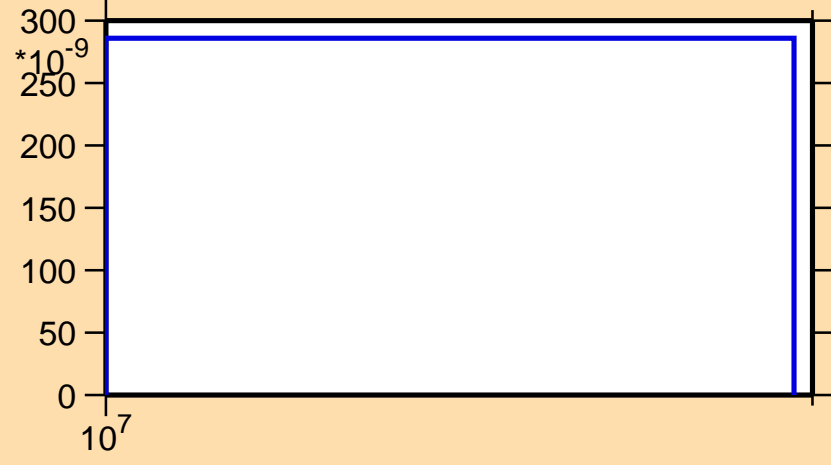
\sigma vs. E for ^{137}\text{Xe}(n,\text{nd})
