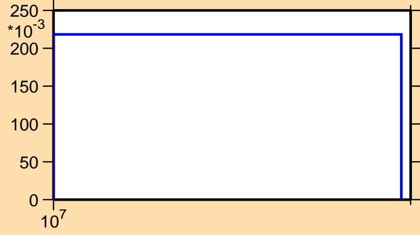
\sigma vs. E for ^{137}\text{Xe}(n,3n)
