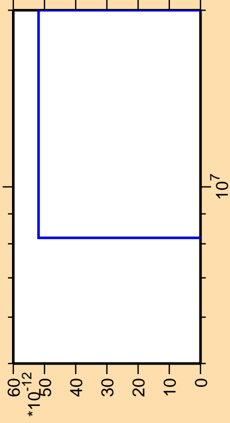
\Delta\sigma/\sigma vs. E for ^{137}\text{Xe}(\text{mt } 11)
