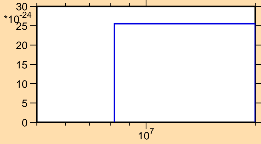
\sigma vs. E for ^{137}\text{Xe}(\text{mt } 11)
