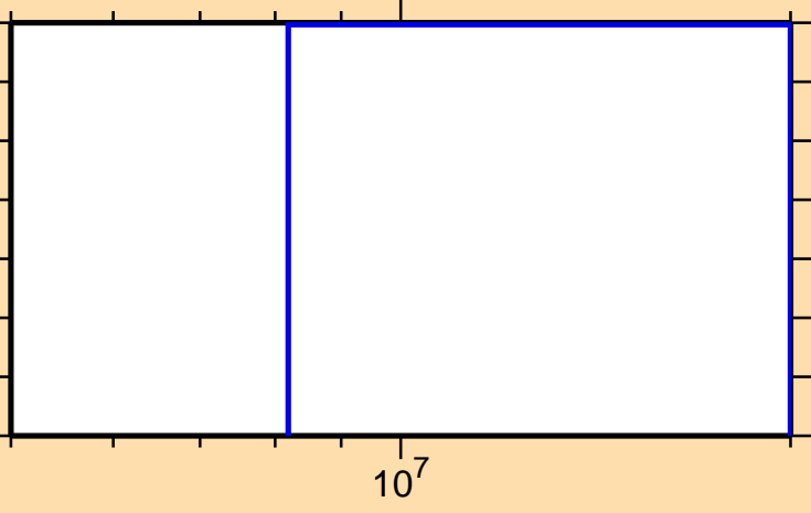
\sigma vs. E for ^{137}\text{Xe}(n,n\alpha)
