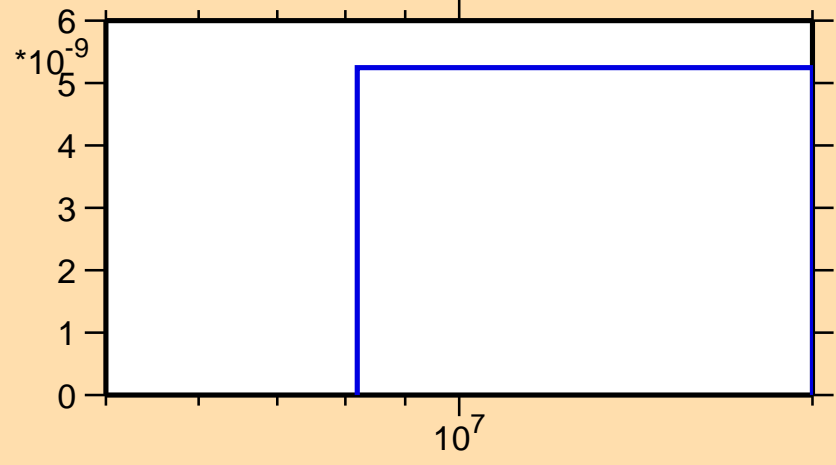
\sigma vs. E for ^{137}\text{Xe}(n,nt)
