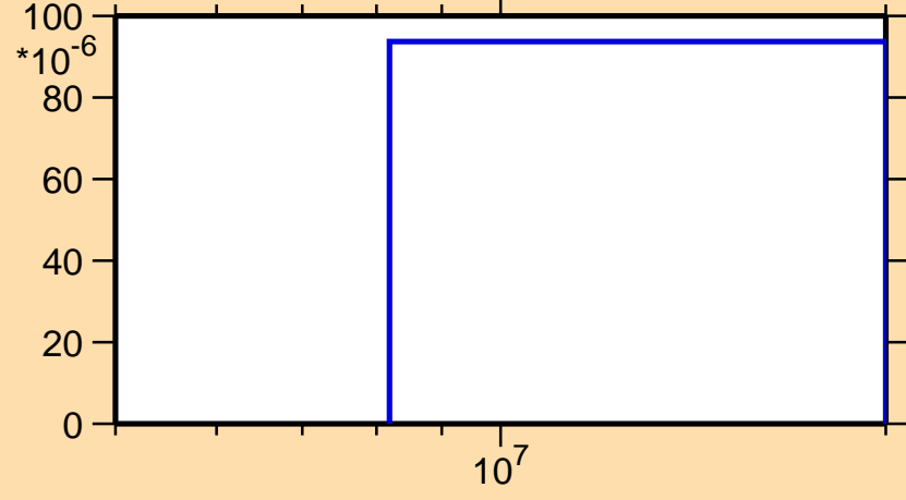
\sigma vs. E for ^{137}\text{Xe}(n,d)
