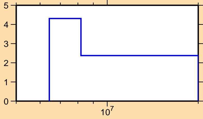
\Delta\sigma/\sigma vs. E for ^{137}\text{Xe}(n,el.)
