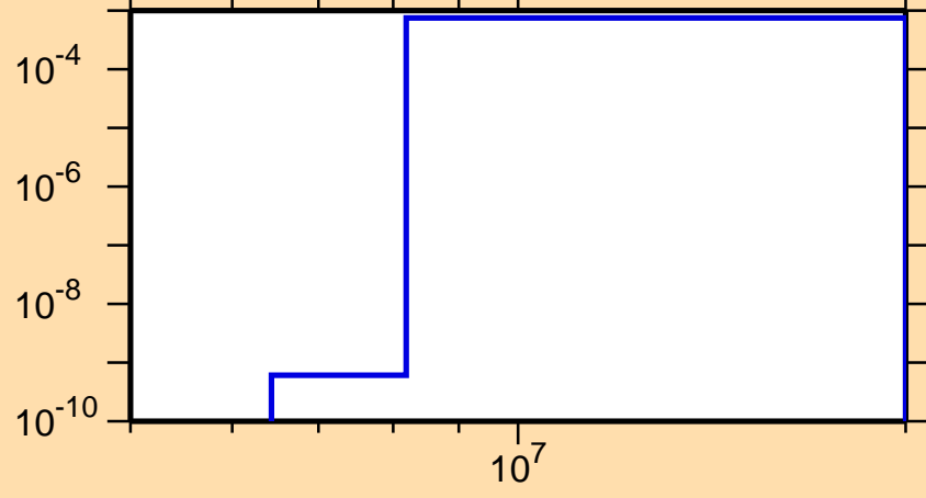
\sigma vs. E for ^{137}\text{Xe}(n,p)
