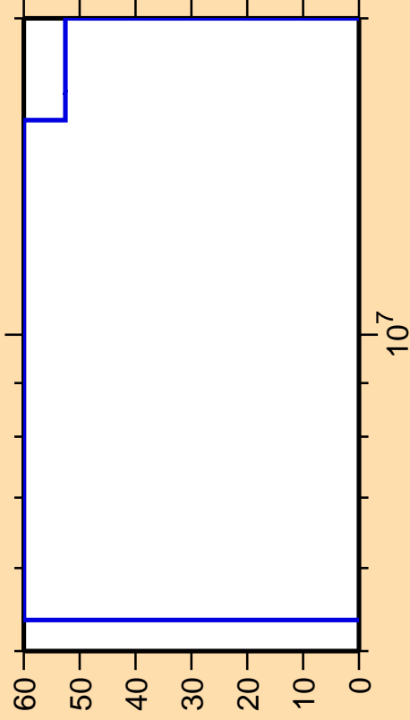
\Delta\sigma/\sigma vs. E for ^{140}\text{Xe}(n,\gamma)
