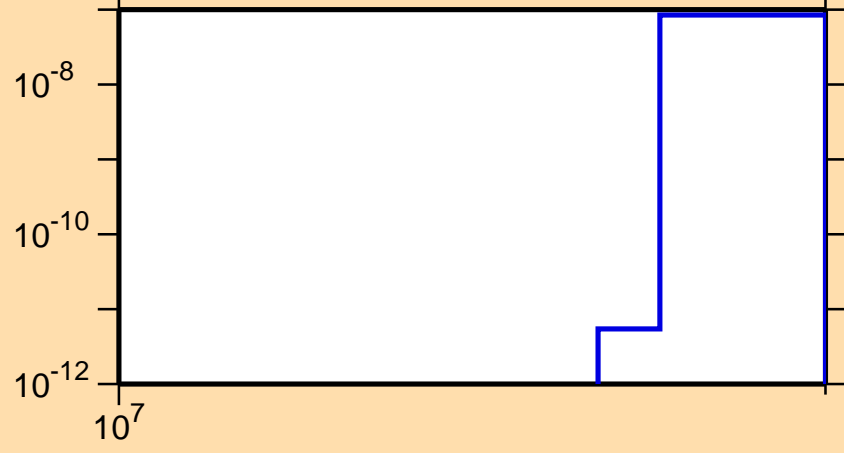
\sigma vs. E for ^{140}\text{Xe}(n,\text{nd})
