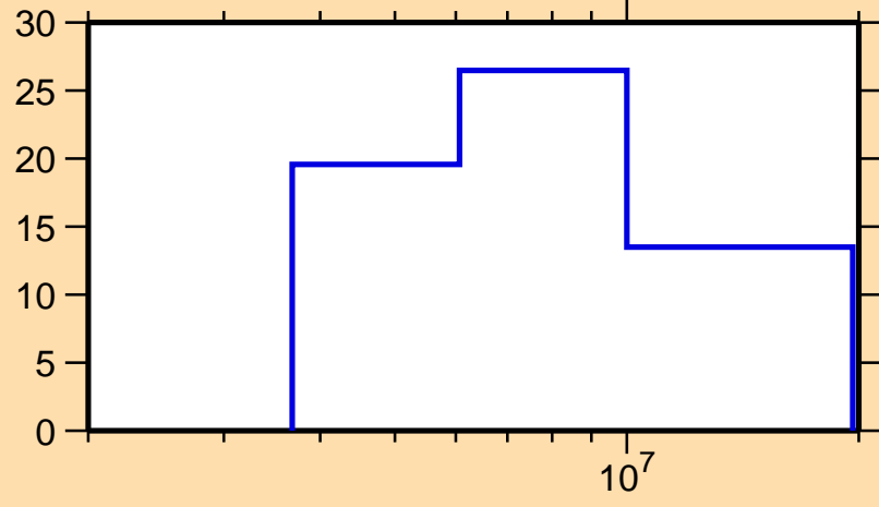
\Delta\sigma/\sigma vs. E for ^{140}\text{Xe}(n,el.)
