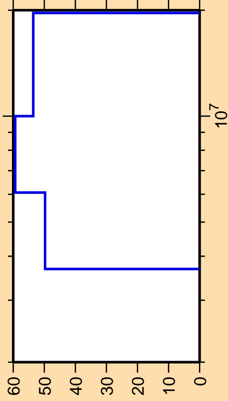
\Delta\sigma/\sigma vs. E for ^{140}\text{Xe}(n,n\text{cont.})
