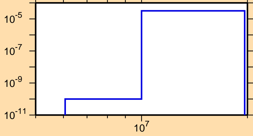
\sigma vs. E for ^{140}\text{Xe}(n,n\alpha)
