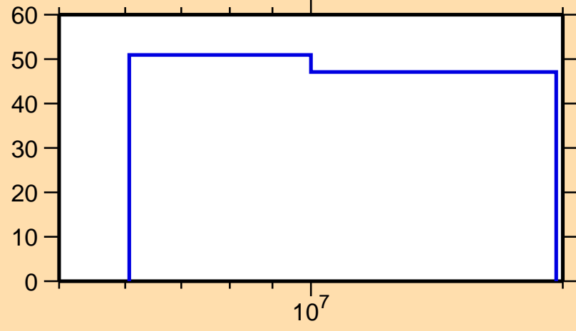
\Delta\sigma/\sigma vs. E for ^{140}\text{Xe}(n,\text{inel.})
