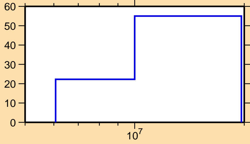
\Delta\sigma/\sigma vs. E for ^{140}\text{Xe}(n,2n)
