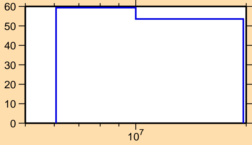
\Delta\sigma/\sigma vs. E for ^{140}\text{Xe}(n,ncont.)
