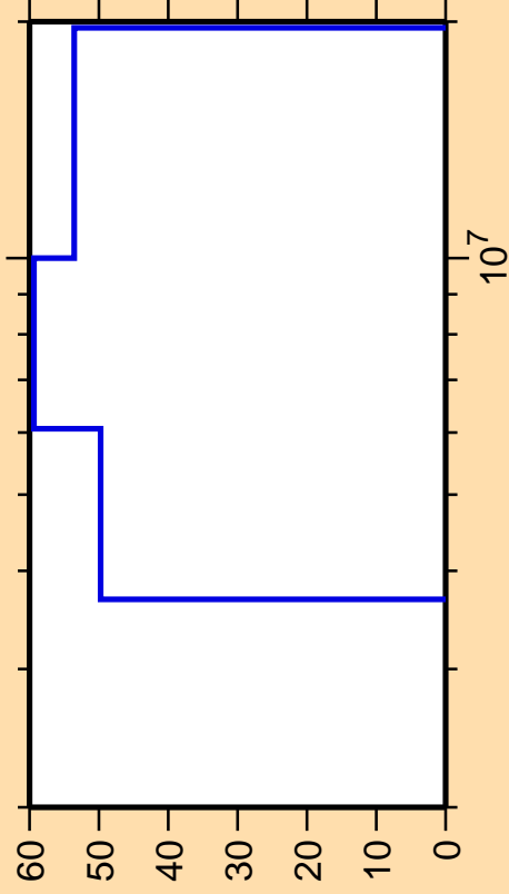
\Delta\sigma/\sigma vs. E for ^{140}\text{Xe}(n,ncont.)
