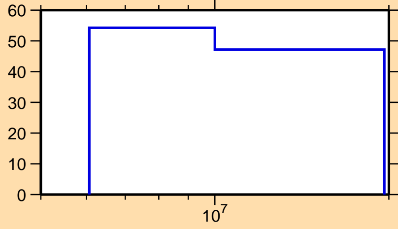
\Delta\sigma/\sigma vs. E for ^{140}\text{Xe}(n,n_1)
