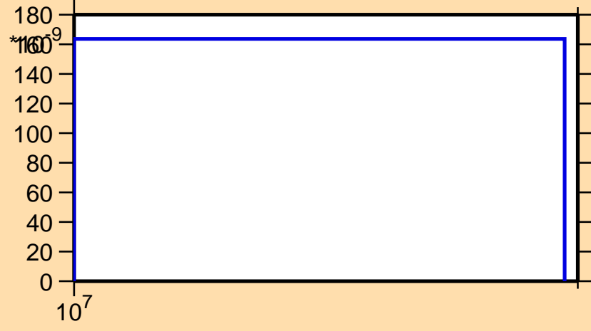
\sigma vs. E for ^{140}\text{Xe}(n,nt)
