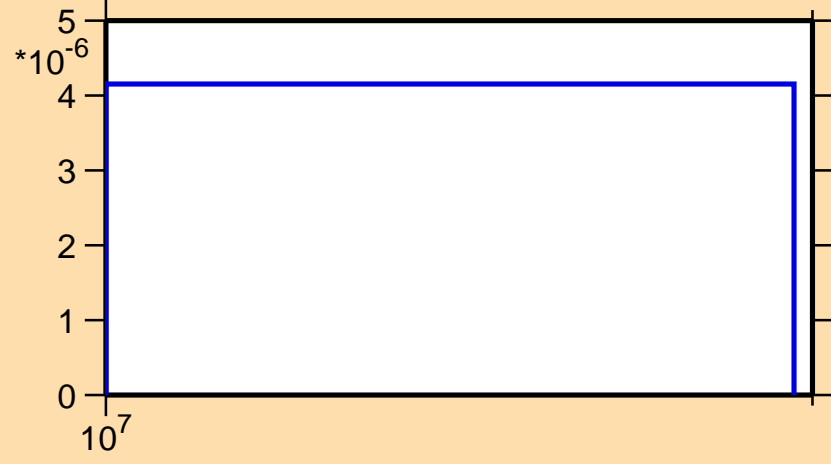
\sigma vs. E for ^{140}\text{Xe}(n,d)
