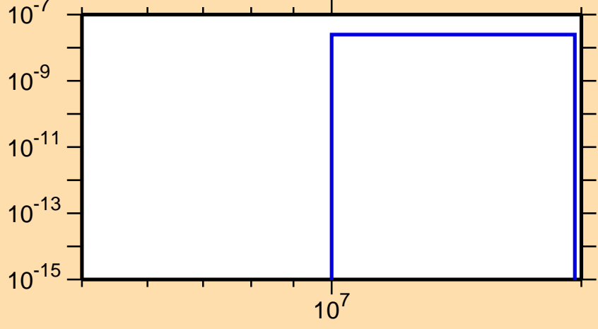
\sigma vs. E for ^{140}\text{Xe}(n,2n\alpha)
