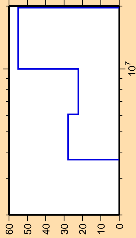
\Delta\sigma/\sigma vs. E for ^{140}\text{Xe}(n,2n)
