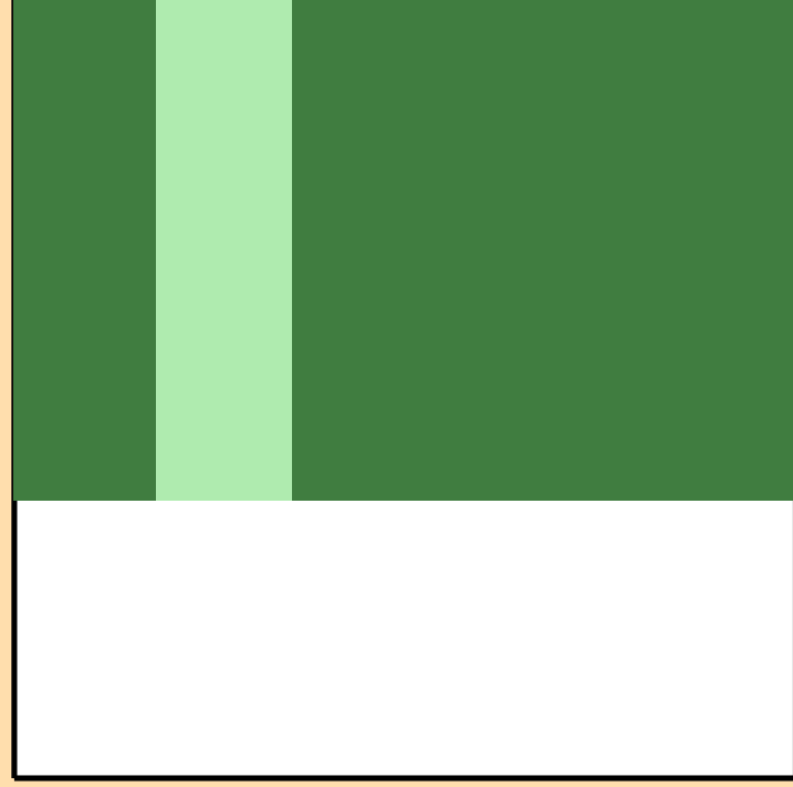
\Delta\sigma/\sigma vs. E for ^{140}\text{Xe}(n,\gamma)
