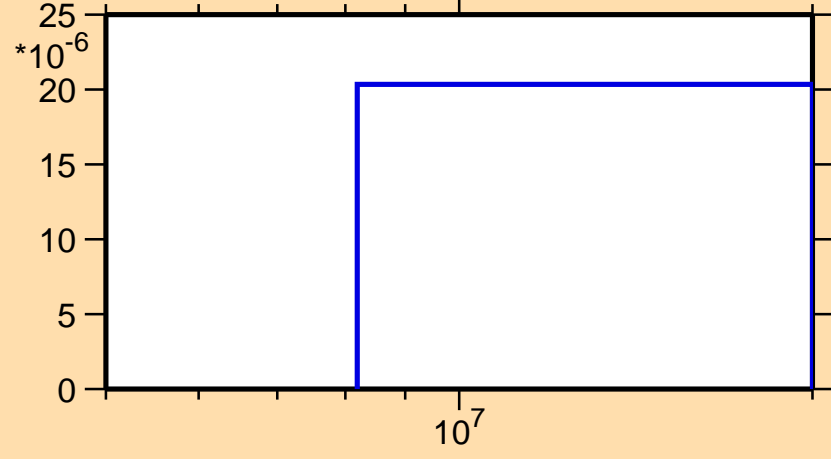
\sigma vs. E for ^{140}\text{Xe}(n,p)
