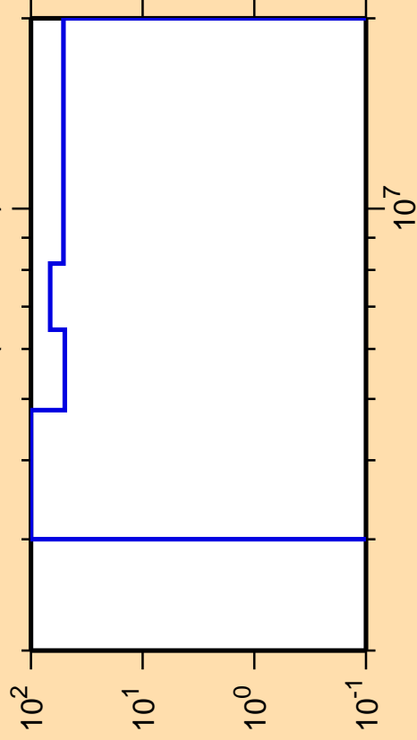
\Delta\sigma/\sigma vs. E for ^{140}\text{Xe}(n,\text{ncont.})
