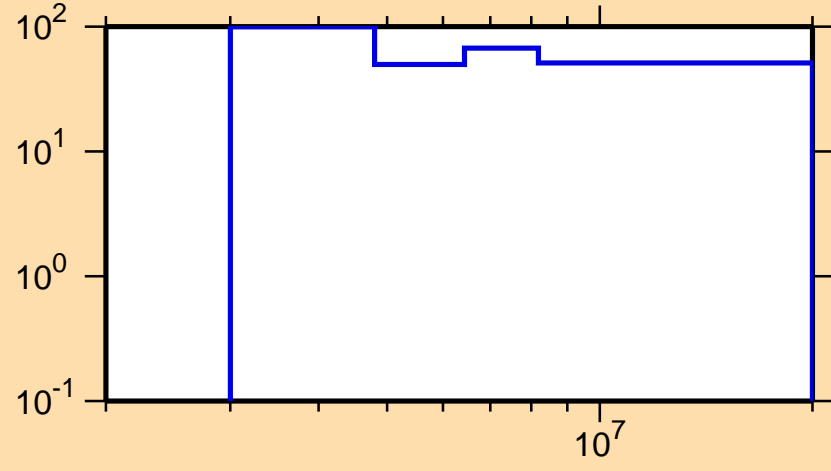
\Delta\sigma/\sigma vs. E for ^{140}\text{Xe}(n,n\text{cont.})
