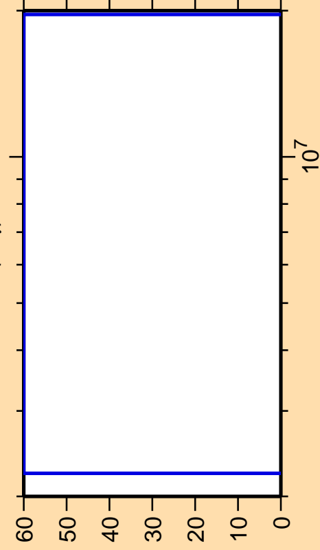
\Delta\sigma/\sigma vs. E for ^{141}\text{Xe}(n,\gamma)
