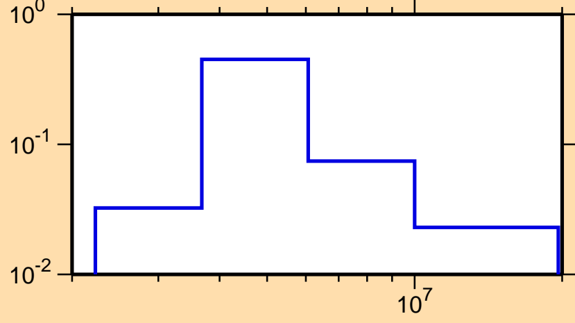
\sigma vs. E for ^{141}\text{Xe}(n,n\text{cont.})
