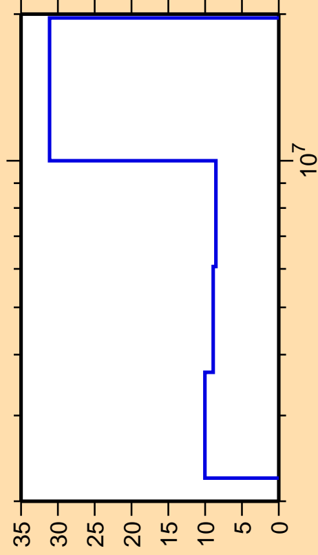
\Delta\sigma/\sigma vs. E for ^{141}\text{Xe}(n,2n)
