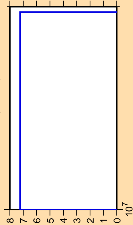
\Delta\sigma/\sigma vs. E for ^{141}\text{Xe}(n,3n\alpha)
