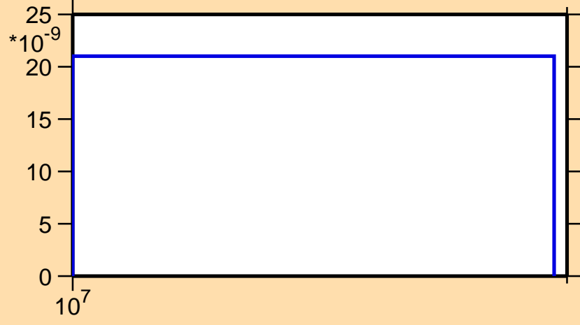
\sigma vs. E for ^{141}\text{Xe}(n,\text{nd})
