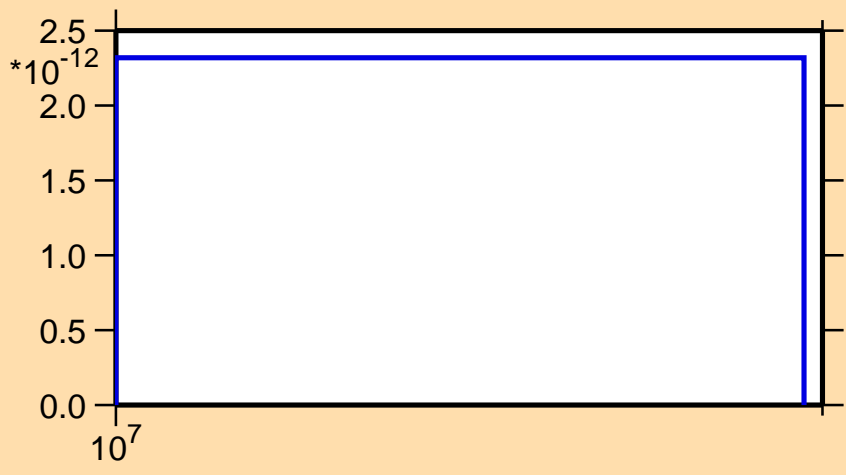
\sigma vs. E for ^{141}\text{Xe}(n,3n\alpha)
