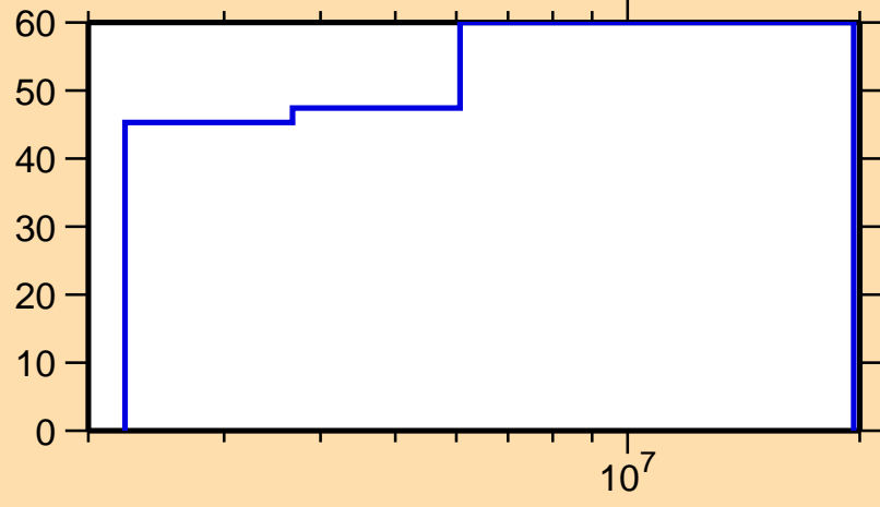
\Delta\sigma/\sigma vs. E for ^{141}\text{Xe}(n,n\text{cont.})
