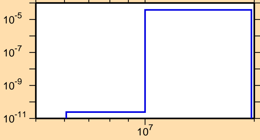
\sigma vs. E for ^{141}\text{Xe}(n,n\alpha)
