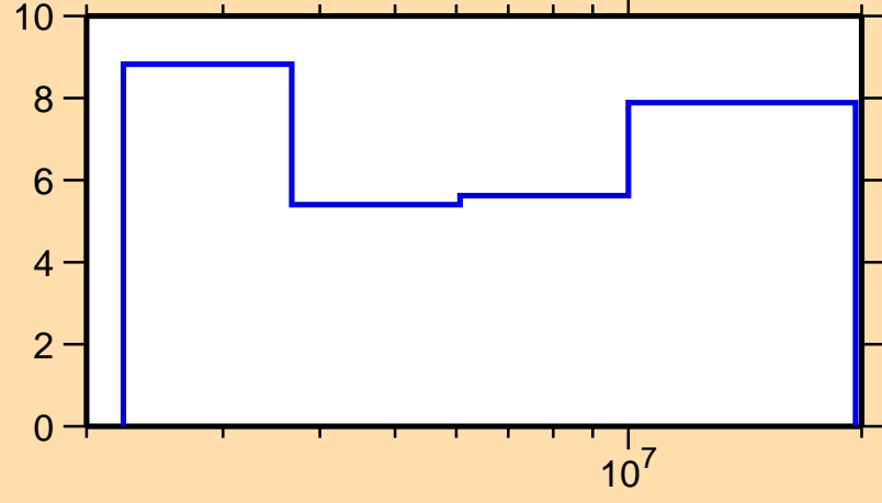
\Delta\sigma/\sigma vs. E for ^{141}\text{Xe}(n,\text{nonel.})
