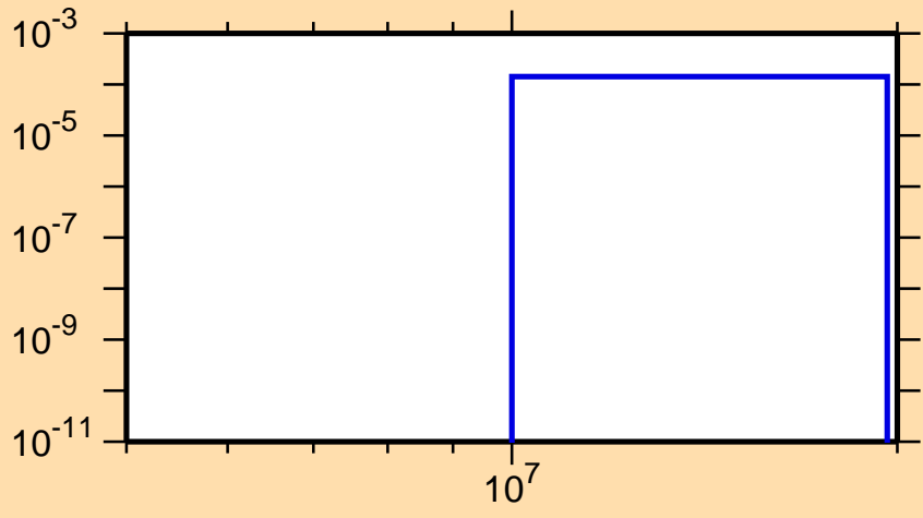
\sigma vs. E for ^{141}\text{Xe}(n,p)
