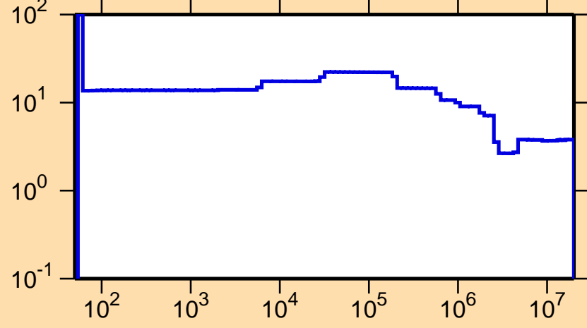
\Delta\sigma/\sigma vs. E for ^{78}\text{Y}(n,\text{nonel.})
