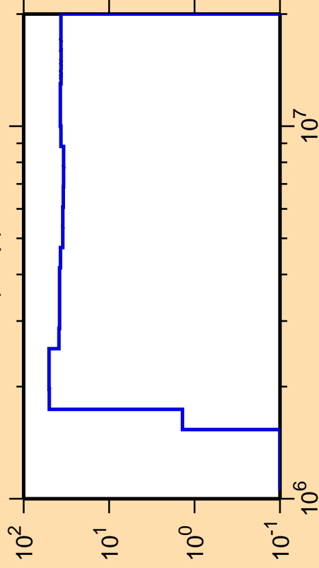
\Delta\sigma/\sigma vs. E for ^{78}\text{Y}(n,np)
