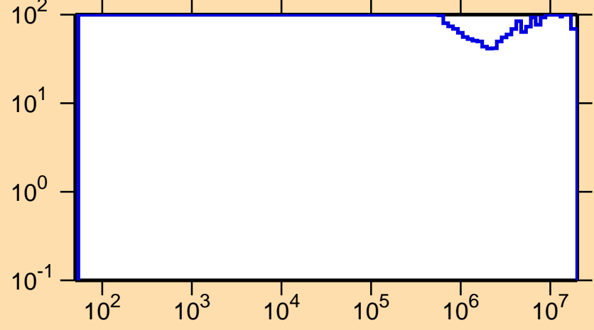
\Delta\sigma/\sigma vs. E for ^{78}\text{Y}(n,n_1)
