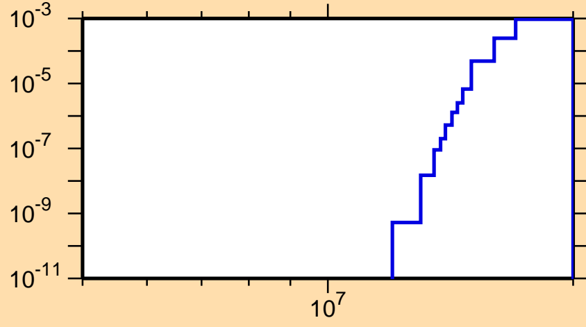
\sigma vs. E for ^{78}\text{Y}(n,pt)
