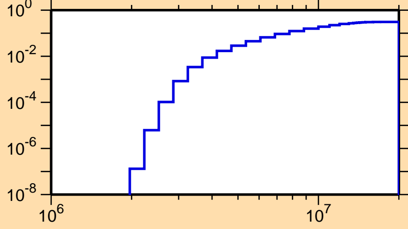
\sigma vs. E for ^{78}\text{Y}(n,np)
