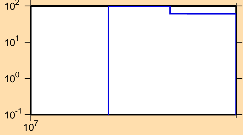
\Delta\sigma/\sigma vs. E for ^{78}\text{Y}(n,2n)
