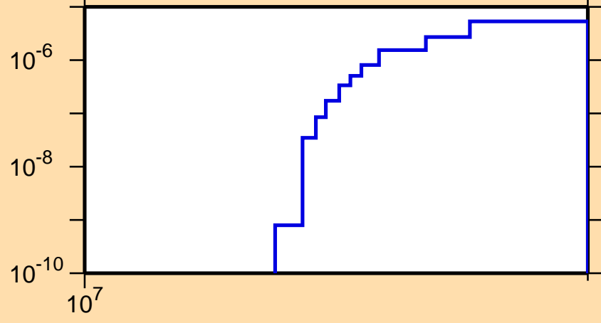
\sigma vs. E for ^{78}\text{Y}(n,2n)
