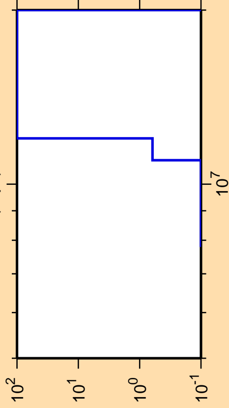
\Delta\sigma/\sigma vs. E for ^{78}\text{Y}(n,pt)
