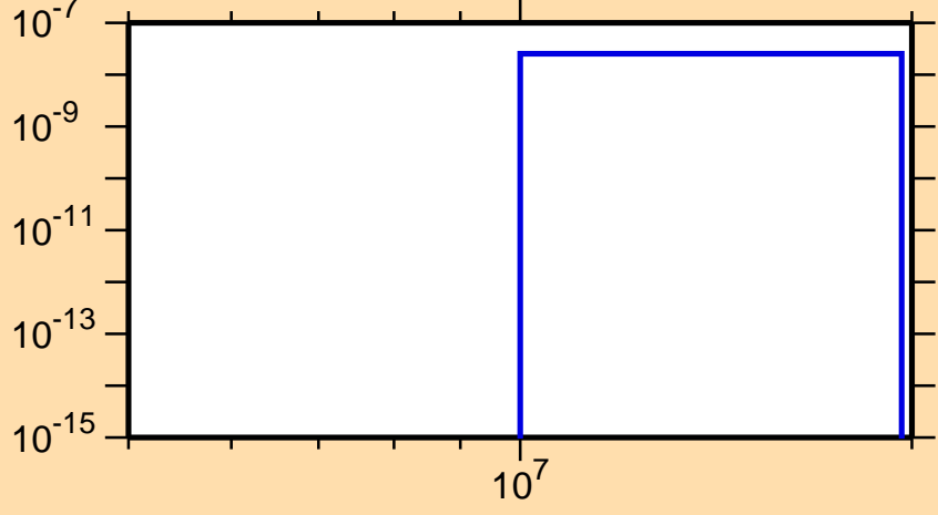
\sigma vs. E for ^{78}\text{Y}(\text{mt117})
