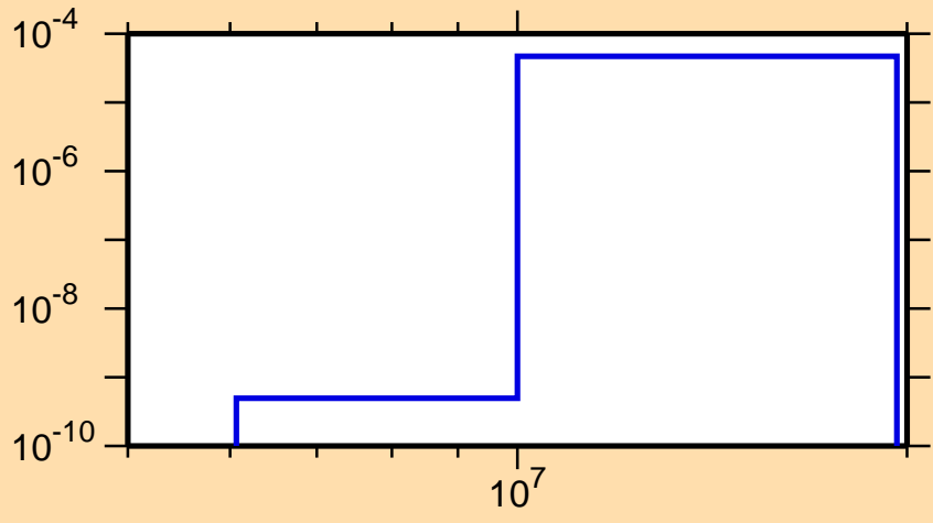
\sigma vs. E for ^{78}\text{Y}(n,n\alpha)
