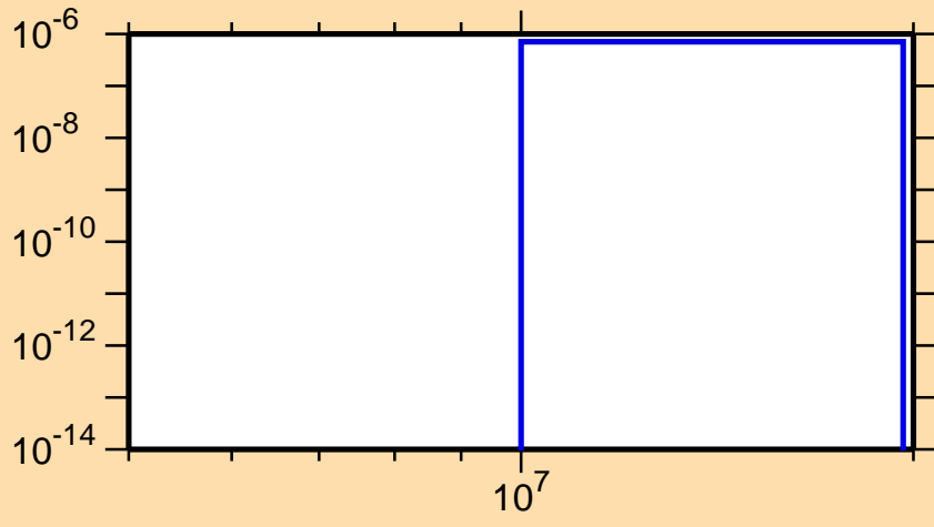
\sigma vs. E for ^{78}\text{Y}(\text{mt } 45)
