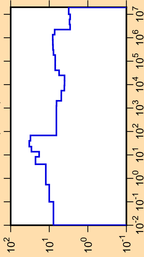
\Delta\sigma/\sigma vs. E for ^{78}\text{Y}(n,\text{tot.})
