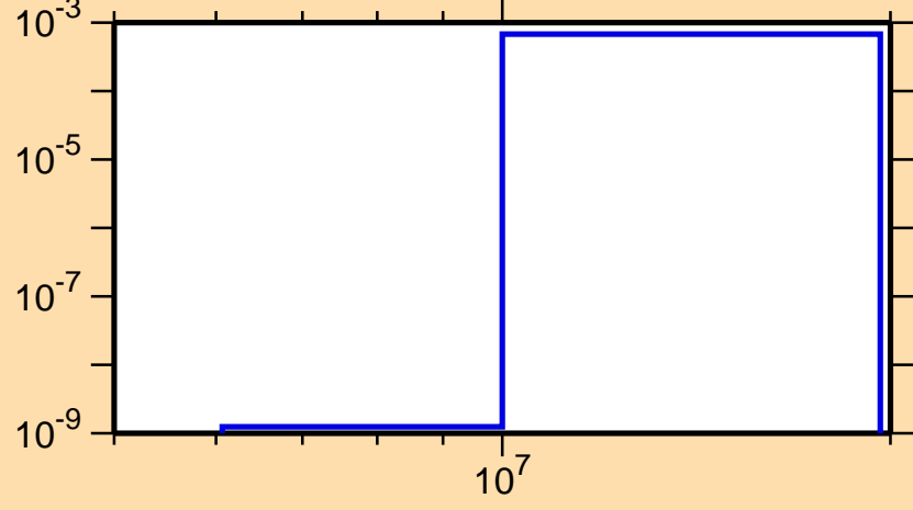
\sigma vs. E for ^{78}\text{Y}(n,t)
