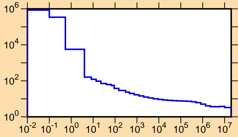
\sigma vs. E for ^{78}\text{Y}(n,\text{tot.})
