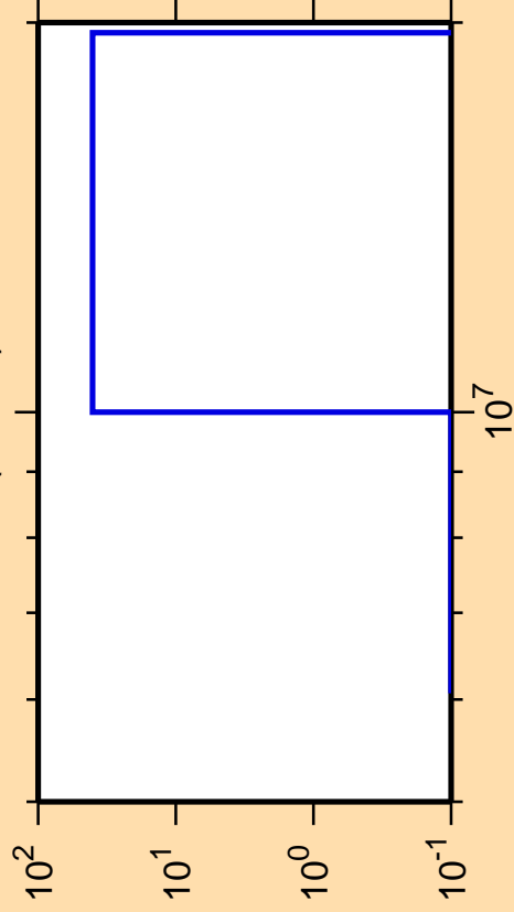
\Delta\sigma/\sigma vs. E for ^{78}\text{Y}(\text{mt } 45)
