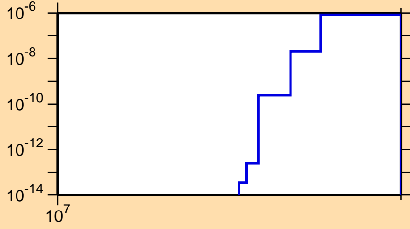
\sigma vs. E for ^{79}\text{Y}(n,nd)
