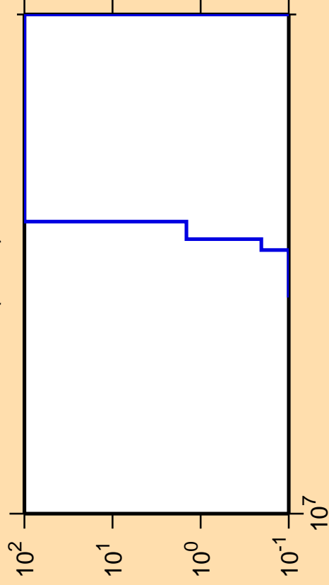
\Delta\sigma/\sigma vs. E for ^{79}\text{Y}(n,nd)
