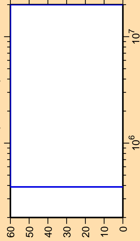
\Delta\sigma/\sigma vs. E for ^{79}\text{Y}(n,n_{\text{cont}})
