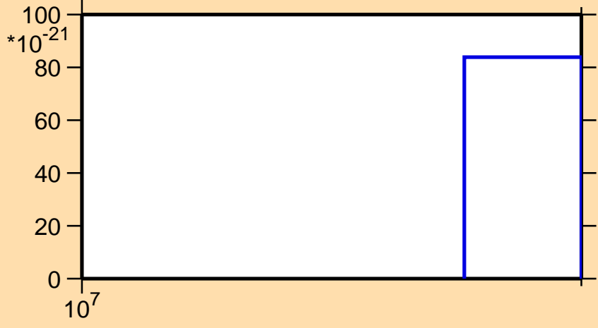
\sigma vs. E for ^{79}\text{Y}(n,nt)
