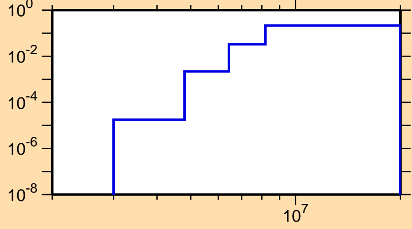
\sigma vs. E for ^{79}\text{Y}(n,np)
