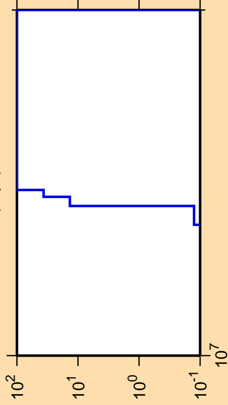
\Delta\sigma/\sigma vs. E for ^{80}\text{Y}(n,pt)
