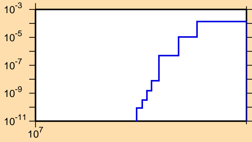
\sigma vs. E for ^{80}\text{Y}(n,pt)
