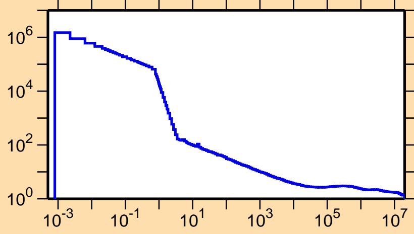
\sigma vs. E for ^{80}\text{Y}(n,\text{nonel.})
