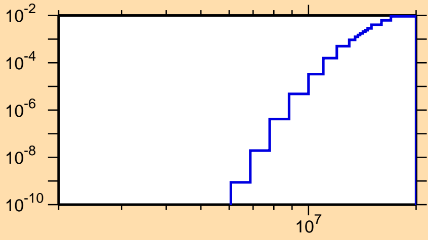
\sigma vs. E for ^{80}\text{Y}(n,\text{He}3)
