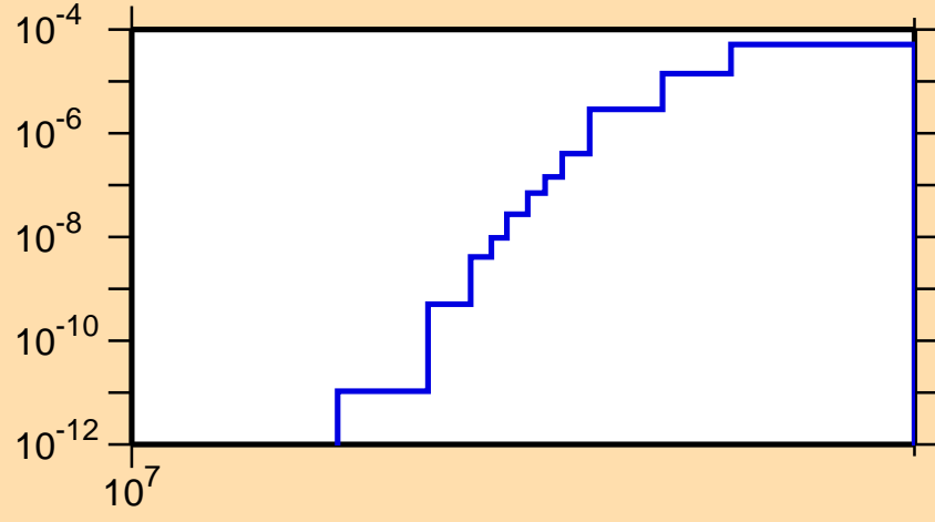
\sigma vs. E for ^{80}\text{Y}(n,nd)
