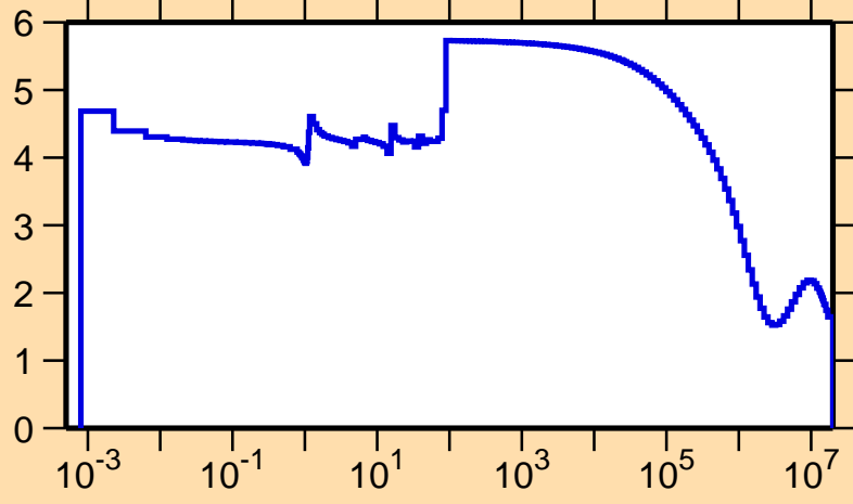
\sigma vs. E for ^{80}\text{Y}(n,\text{el.})
