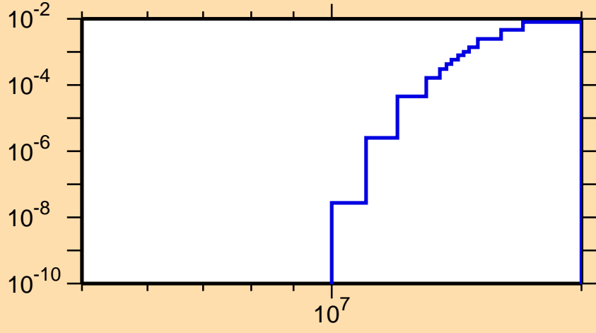
\sigma vs. E for ^{80}\text{Y}(n,\text{pd})
