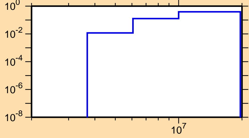
\sigma vs. E for ^{80}\text{Y}(n,np)
