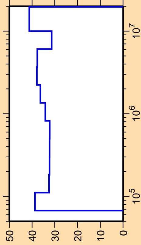
\Delta\sigma/\sigma vs. E for ^{80}\text{Y}(n,n_3)
