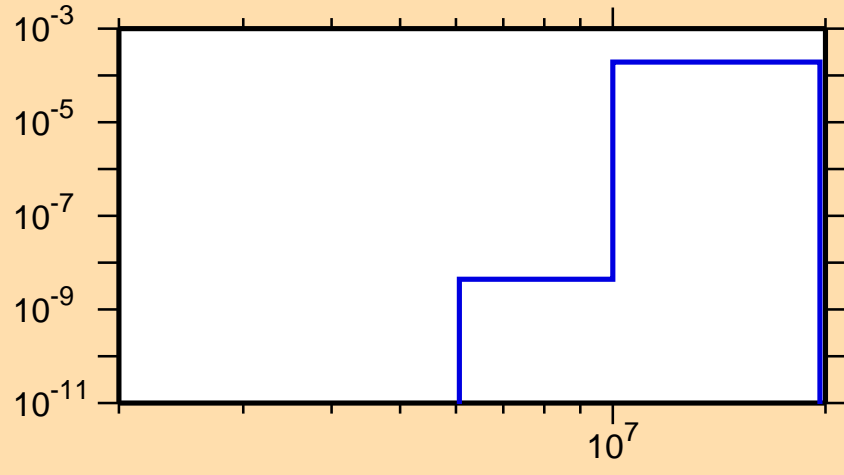
\sigma vs. E for ^{81}\text{Y}(n,\text{He}3)
