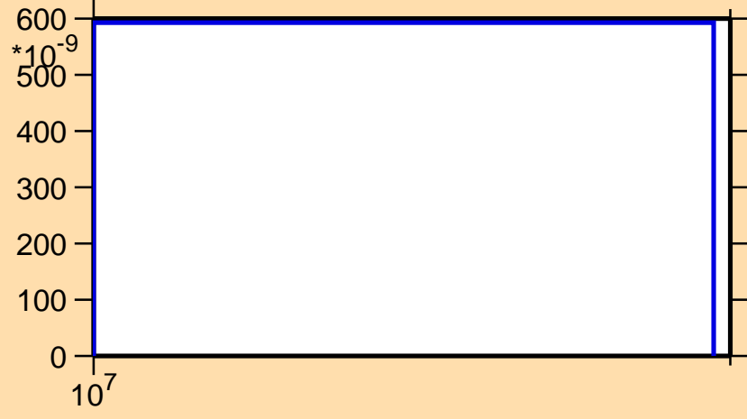
\sigma vs. E for ^{81}\text{Y} (mt 45)
