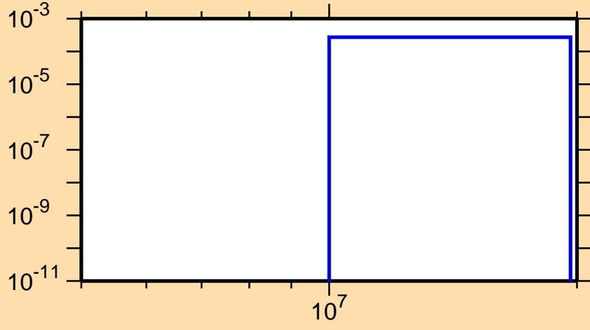
\sigma vs. E for ^{81}\text{Y}(n,\text{pd})
