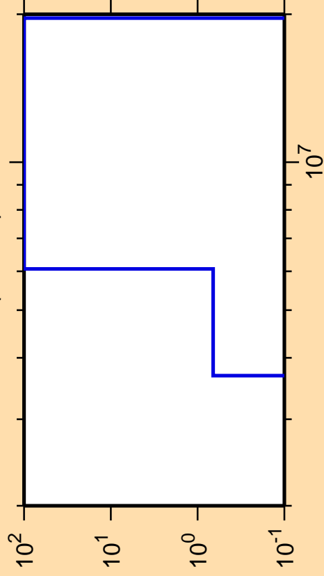
\Delta\sigma/\sigma vs. E for ^{81}\text{Y}(n,\text{He}3)
