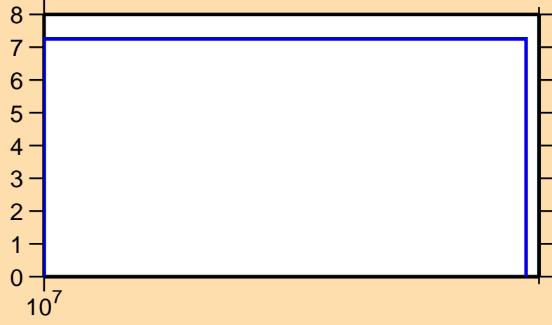
\Delta\sigma/\sigma vs. E for ^{81}\text{Y}(n,\text{nonel.})
