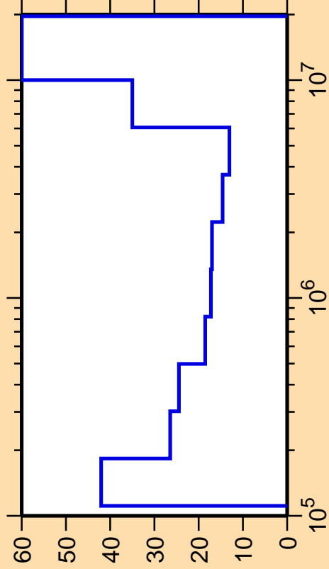
\Delta\sigma/\sigma vs. E for ^{81}\text{Y}(n,p)
