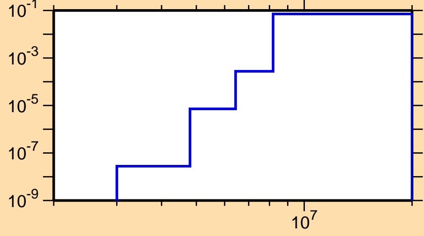
\sigma vs. E for ^{81}\text{Y}(n,p\alpha)
