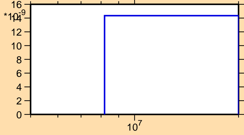
\sigma vs. E for ^{81}\text{Y}(n,nd)
