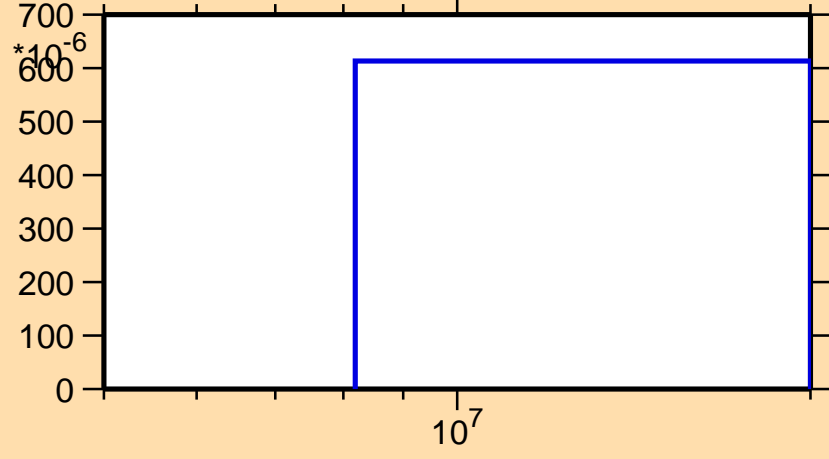
\sigma vs. E for ^{81}\text{Y}(n,2n)
