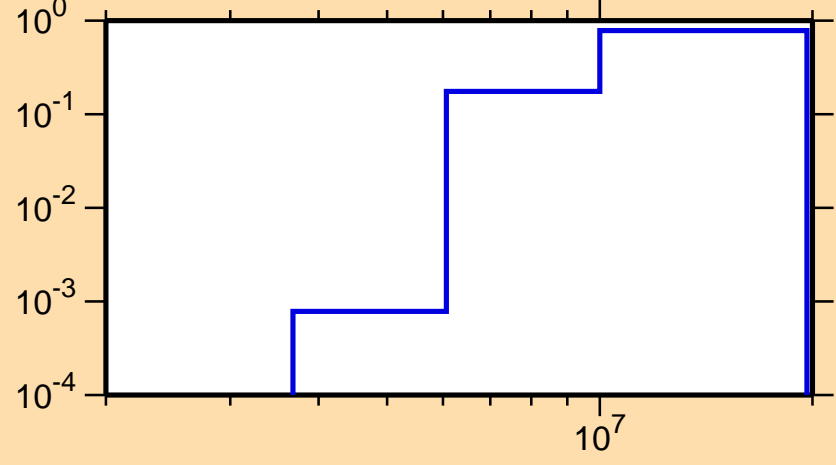
\sigma vs. E for ^{82}\text{Y}(n,np)
