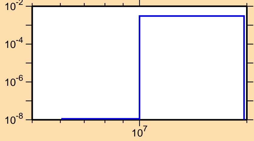
\sigma vs. E for ^{82}\text{Y}(n,n\alpha)
