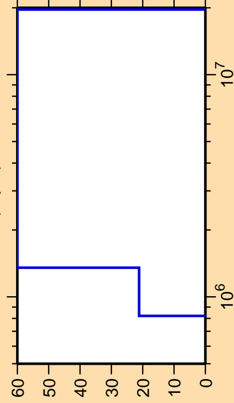
\Delta\sigma/\sigma vs. E for ^{82}\text{Y}(n,p\alpha)
