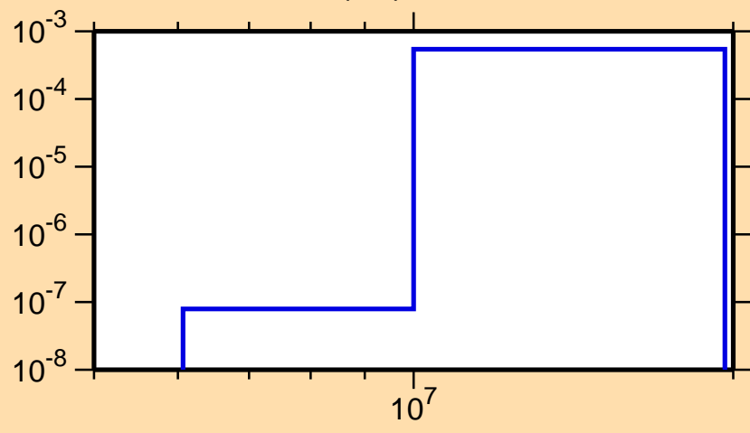
\sigma vs. E for ^{82}\text{Y}(n,t)
