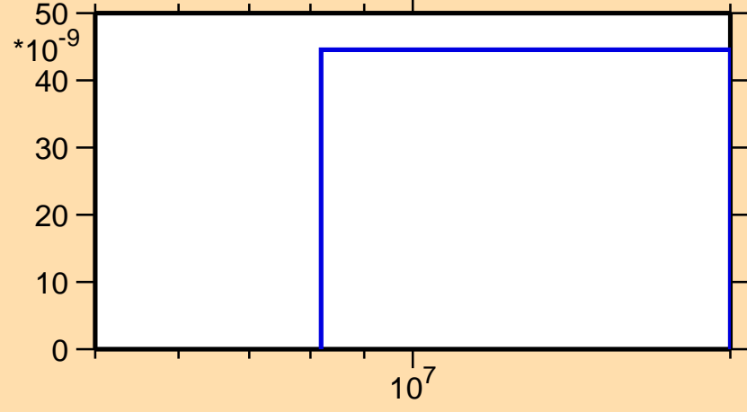
\sigma vs. E for ^{83}\text{Y}(n,nd)
