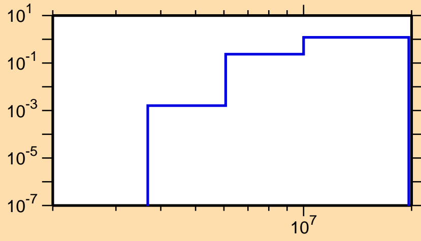
\sigma vs. E for ^{83}\text{Y}(n,np)
