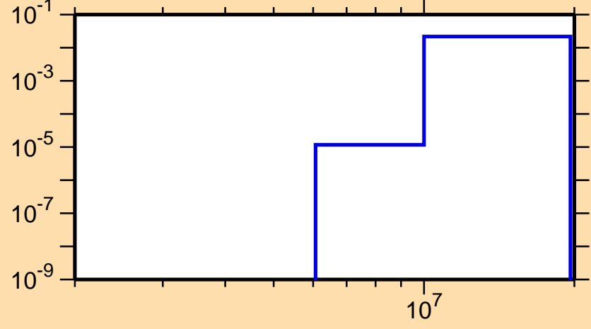
\sigma vs. E for ^{83}\text{Y}(n,p\alpha)
