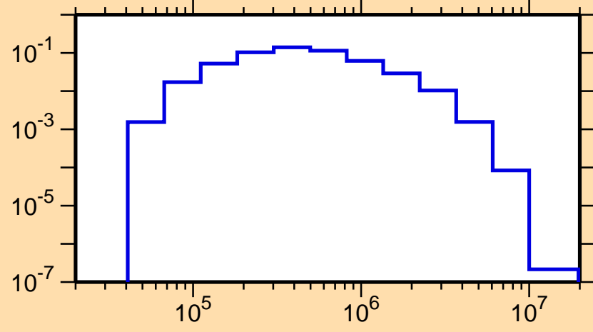
\sigma vs. E for ^{83}\text{Y}(n,n_3)
