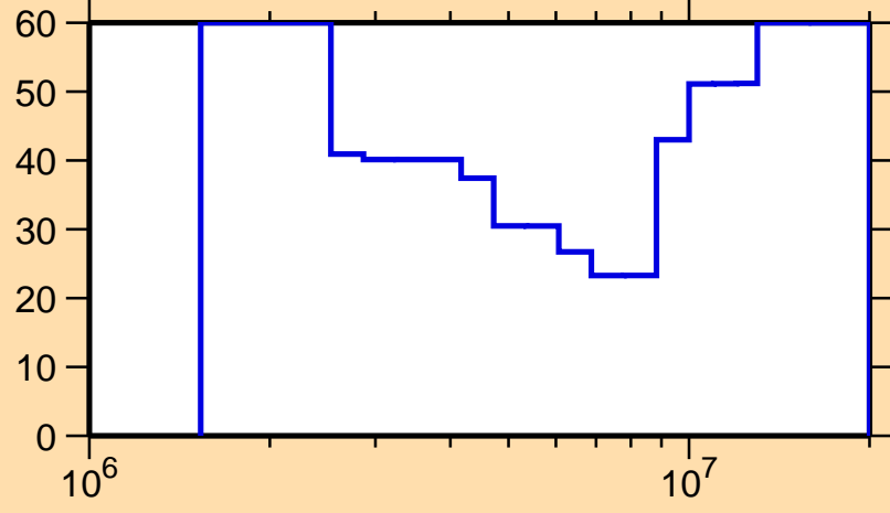
\Delta\sigma/\sigma vs. E for ^{84}\text{Y}(n,ncont.)
