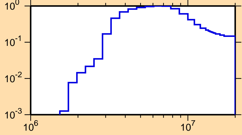
\sigma vs. E for ^{84}\text{Y}(n,n\text{cont.})
