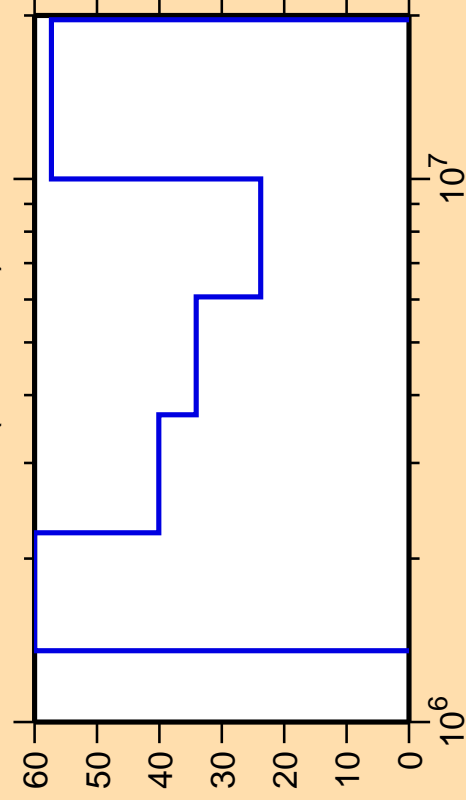
\Delta\sigma/\sigma vs. E for ^{84}\text{Y}(n,n\text{cont.})
