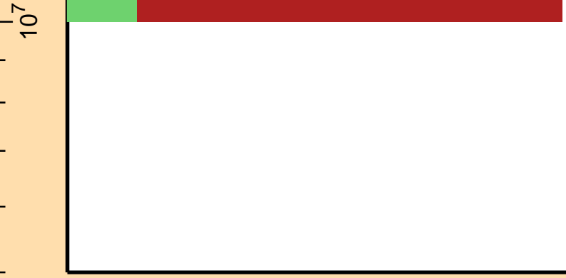
Correlation Matrix
