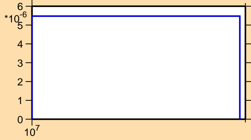
\sigma vs. E for ^{84}\text{Y}(n,nd)
