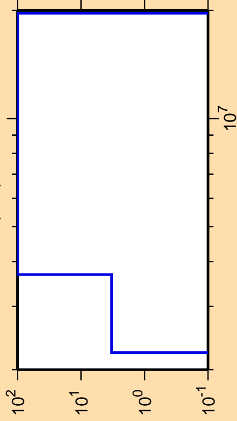
\Delta\sigma/\sigma vs. E for ^{84}\text{Y}(n,d)
