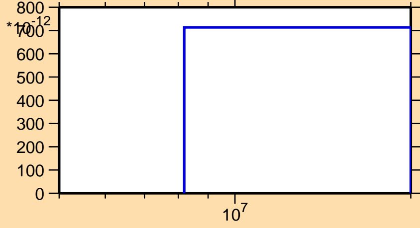
\sigma vs. E for ^{84}\text{Y}(n,pt)
