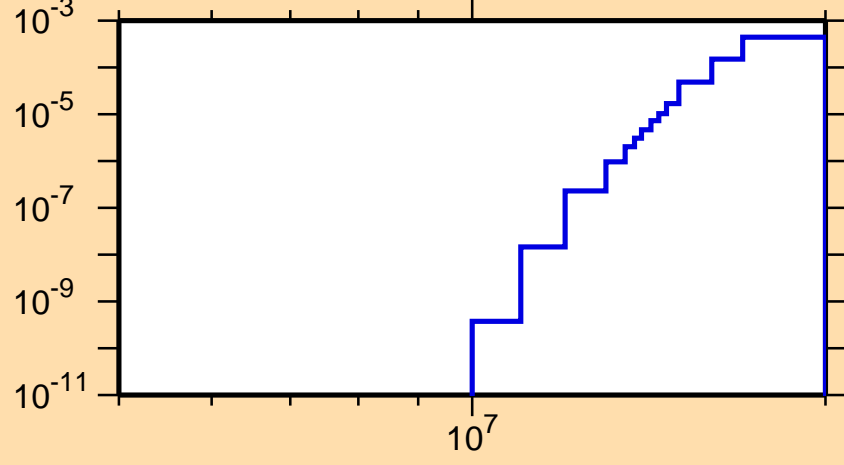
\sigma vs. E for ^{84}\text{Y}(n,\text{He}3)
