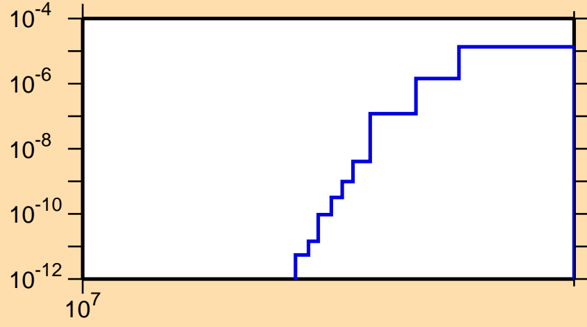
\sigma vs. E for ^{84}\text{Y}(n,pd)
