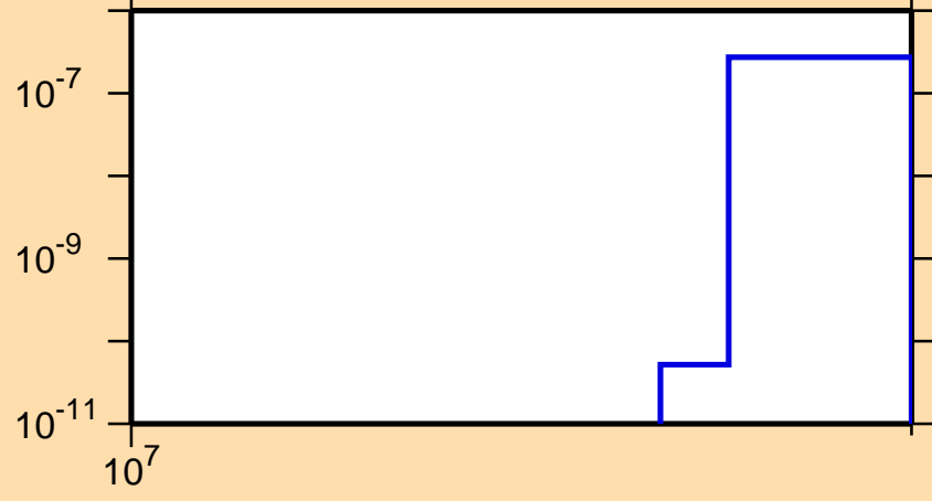
\sigma vs. E for ^{84}\text{Y}(n,\text{pt})
