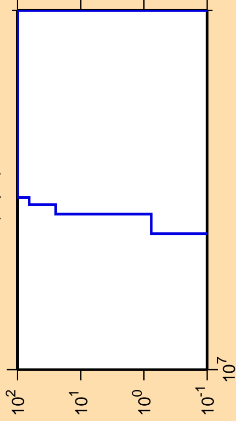
\Delta\sigma/\sigma vs. E for ^{84}\text{Y}(n,pd)
