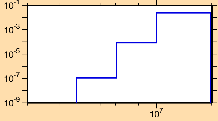
\sigma vs. E for ^{84}\text{Y}(n,p\alpha)
