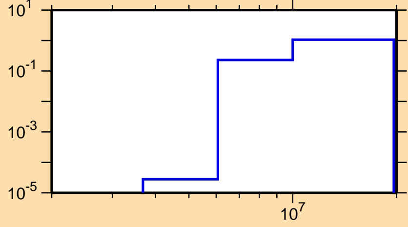
\sigma vs. E for ^{84}\text{Y}(n,np)
