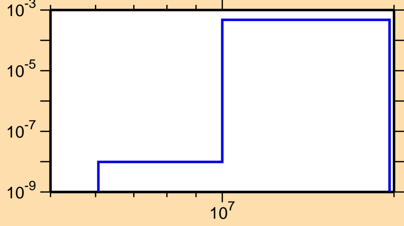
\sigma vs. E for ^{84}\text{Y}(n,t)
