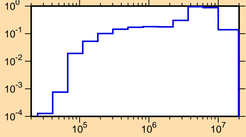
\sigma vs. E for ^{84}\text{Y}(n,\text{inel.})
