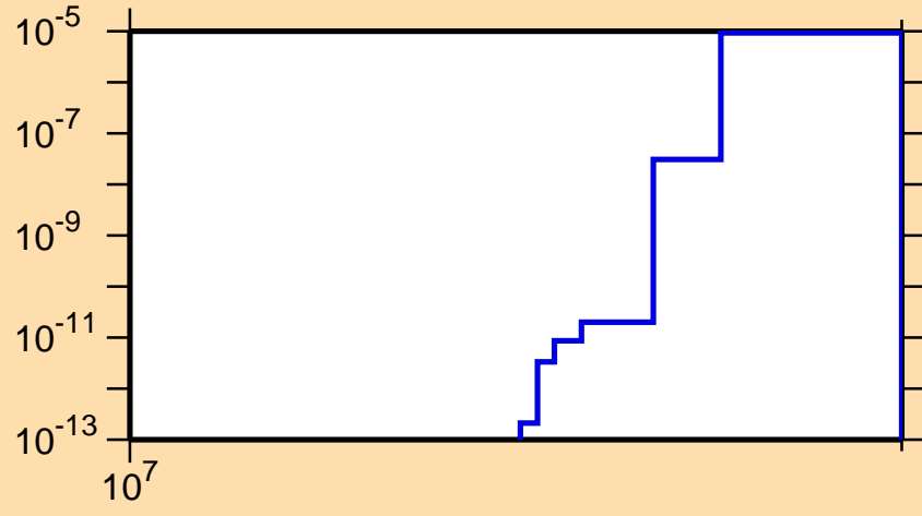
\sigma vs. E for ^{85}\text{Y}(n,nd)
