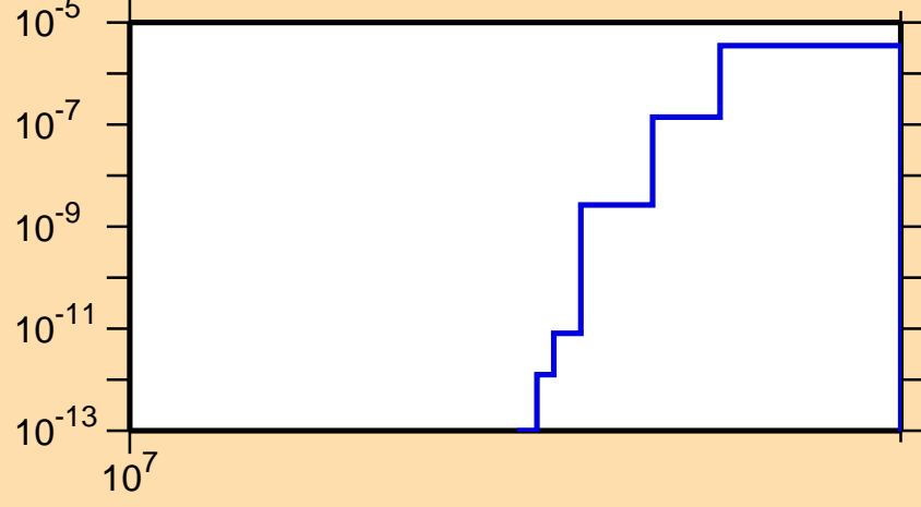
\sigma vs. E for ^{85}\text{Y}(n,pd)
