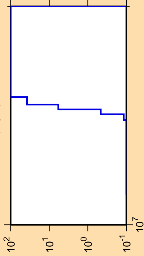
\Delta\sigma/\sigma vs. E for ^{85}\text{Y}(n,pd)
